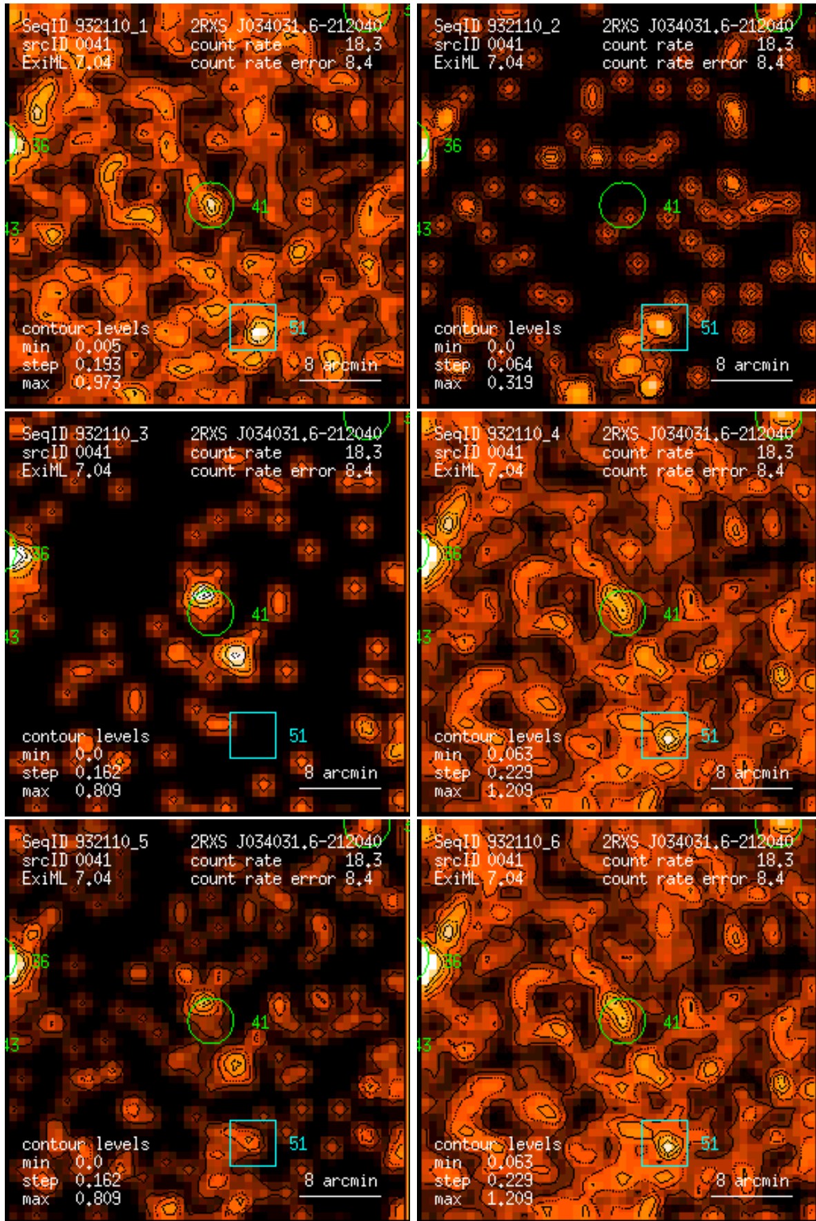
Figure 41: RASS 932110: detection 0041: band rate images, Gaussian filter: (1) PSPC channels 11 – 41, (2) 52 – 90, (3) 91 – 201, (4) 11 – 235, (5) 52 – 201, (6) 11 – 201. Broad band rates in counts/ks. Band rate contour levels in counts/ks/arcmin 2 .
