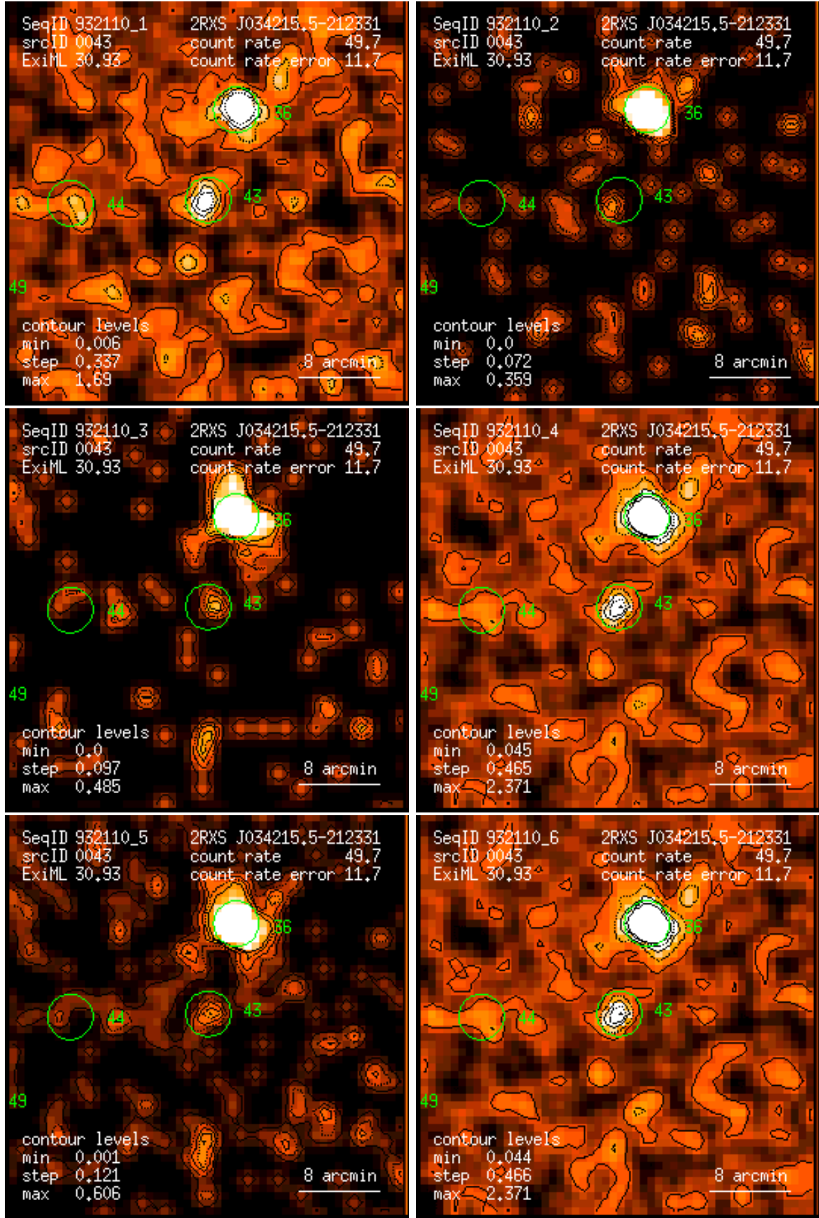
Figure 43: RASS 932110: detection 0043: band rate images, Gaussian filter: (1) PSPC channels 11 – 41, (2) 52 – 90, (3) 91 – 201, (4) 11 – 235, (5) 52 – 201, (6) 11 – 201. Broad band rates in counts/ks. Band rate contour levels in counts/ks/arcmin 2 .
