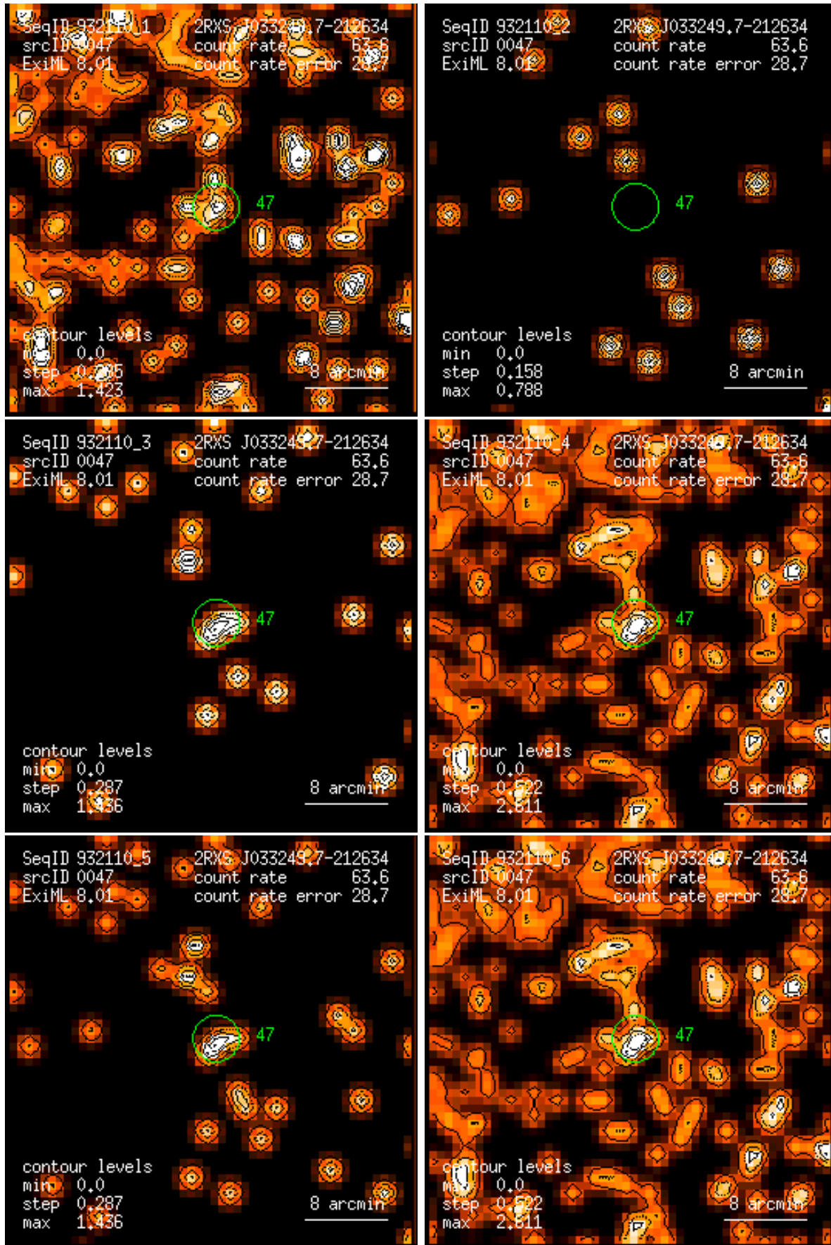
Figure 47: RASS 932110: detection 0047: band rate images, Gaussian filter: (1) PSPC channels 11 – 41, (2) 52 – 90, (3) 91 – 201, (4) 11 – 235, (5) 52 – 201, (6) 11 – 201. Broad band rates in counts/ks. Band rate contour levels in counts/ks/arcmin 2 .
