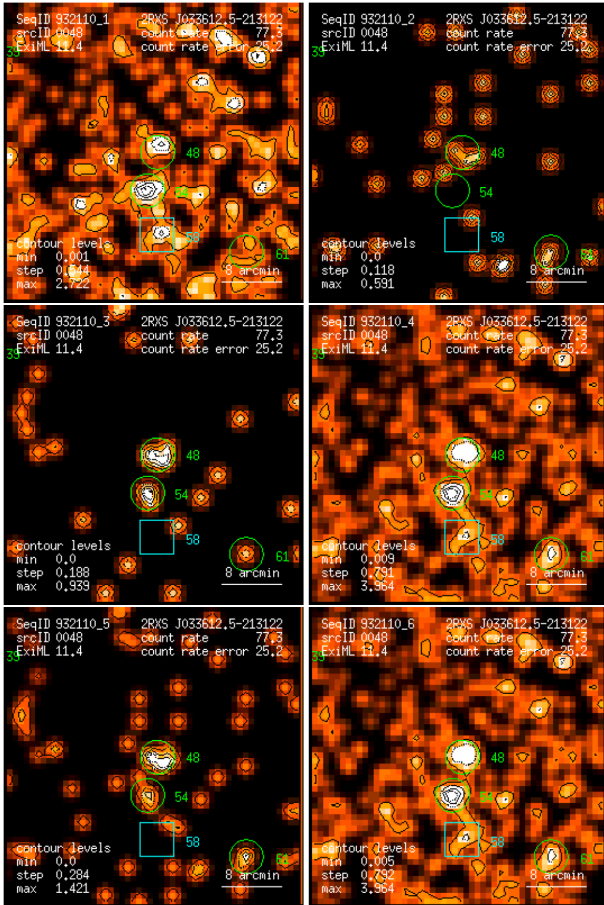
Figure 48: RASS 932110: detection 0048: band rate images, Gaussian filter: (1) PSPC channels 11 – 41, (2) 52 – 90, (3) 91 – 201, (4) 11 – 235, (5) 52 – 201, (6) 11 – 201. Broad band rates in counts/ks. Band rate contour levels in counts/ks/arcmin 2 .
