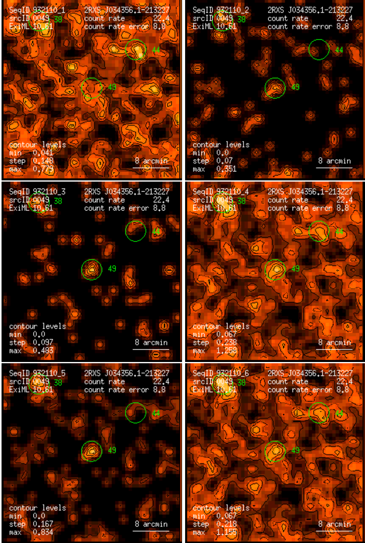
Figure 49: RASS 932110: detection 0049: band rate images, Gaussian filter: (1) PSPC channels 11 – 41, (2) 52 – 90, (3) 91 – 201, (4) 11 – 235, (5) 52 – 201, (6) 11 – 201. Broad band rates in counts/ks. Band rate contour levels in counts/ks/arcmin 2 .
