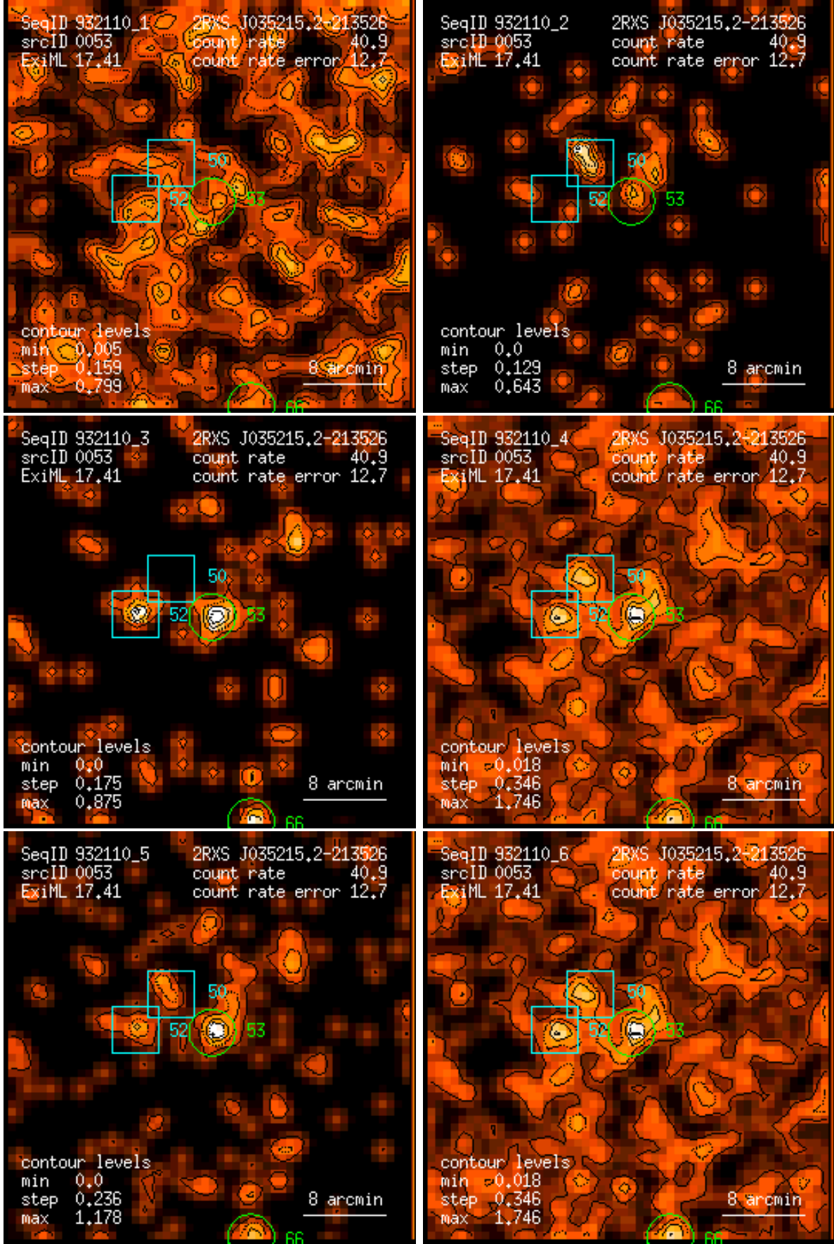
Figure 53: RASS 932110: detection 0053: band rate images, Gaussian filter: (1) PSPC channels 11 – 41, (2) 52 – 90, (3) 91 – 201, (4) 11 – 235, (5) 52 – 201, (6) 11 – 201. Broad band rates in counts/ks. Band rate contour levels in counts/ks/arcmin 2 .
