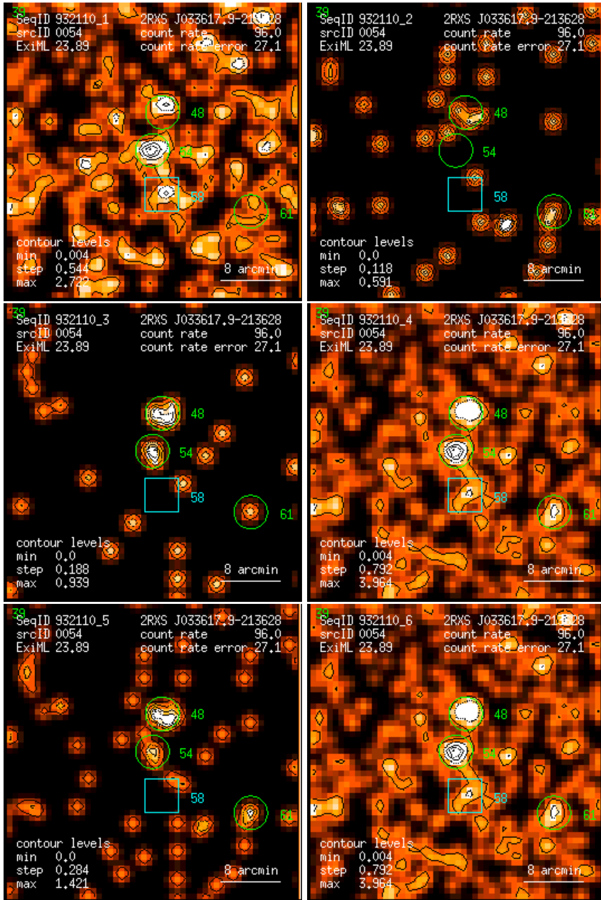
Figure 54: RASS 932110: detection 0054: band rate images, Gaussian filter: (1) PSPC channels 11 – 41, (2) 52 – 90, (3) 91 – 201, (4) 11 – 235, (5) 52 – 201, (6) 11 – 201. Broad band rates in counts/ks. Band rate contour levels in counts/ks/arcmin 2 .
