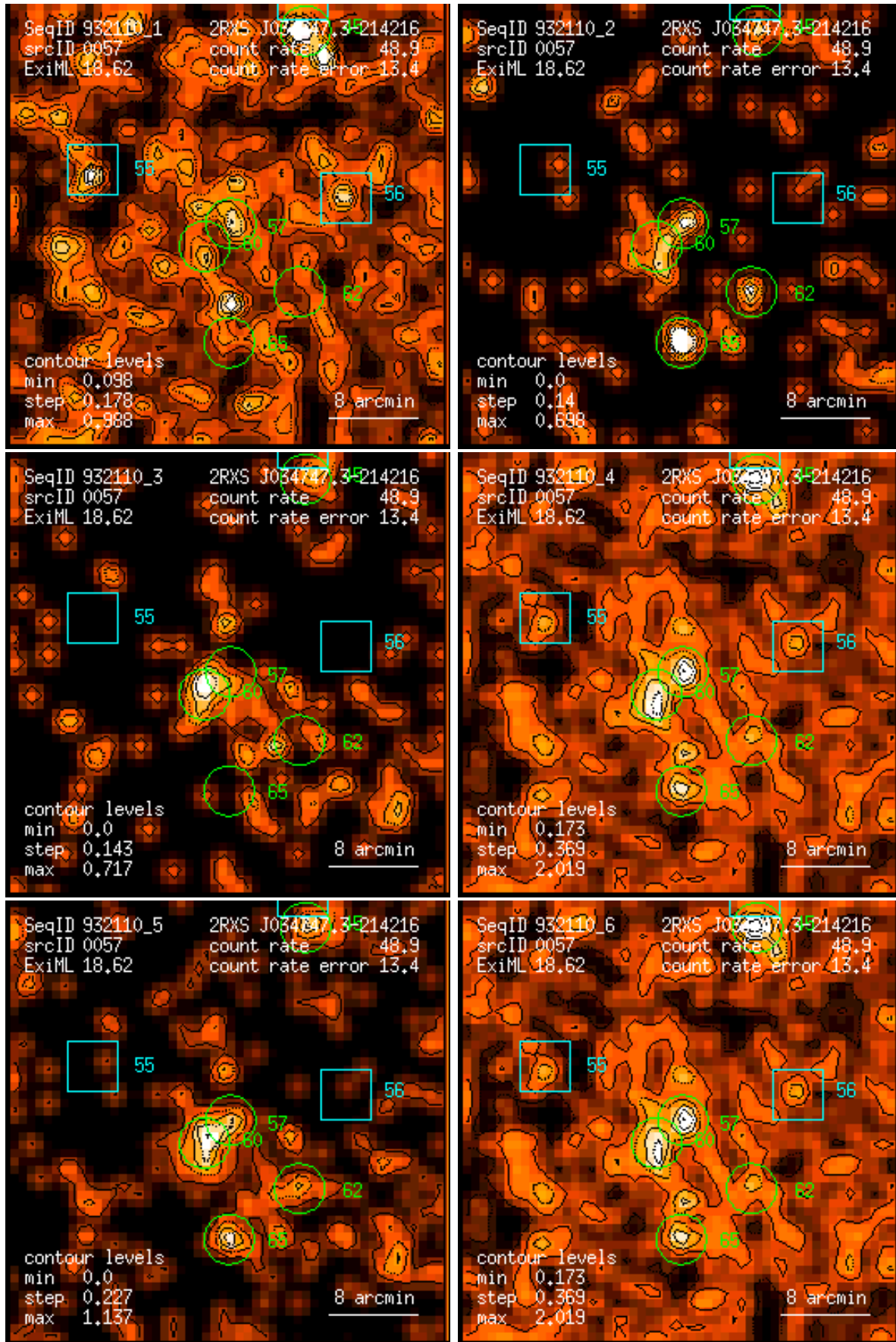
Figure 57: RASS 932110: detection 0057: band rate images, Gaussian filter: (1) PSPC channels 11 – 41, (2) 52 – 90, (3) 91 – 201, (4) 11 – 235, (5) 52 – 201, (6) 11 – 201. Broad band rates in counts/ks. Band rate contour levels in counts/ks/arcmin 2 .
