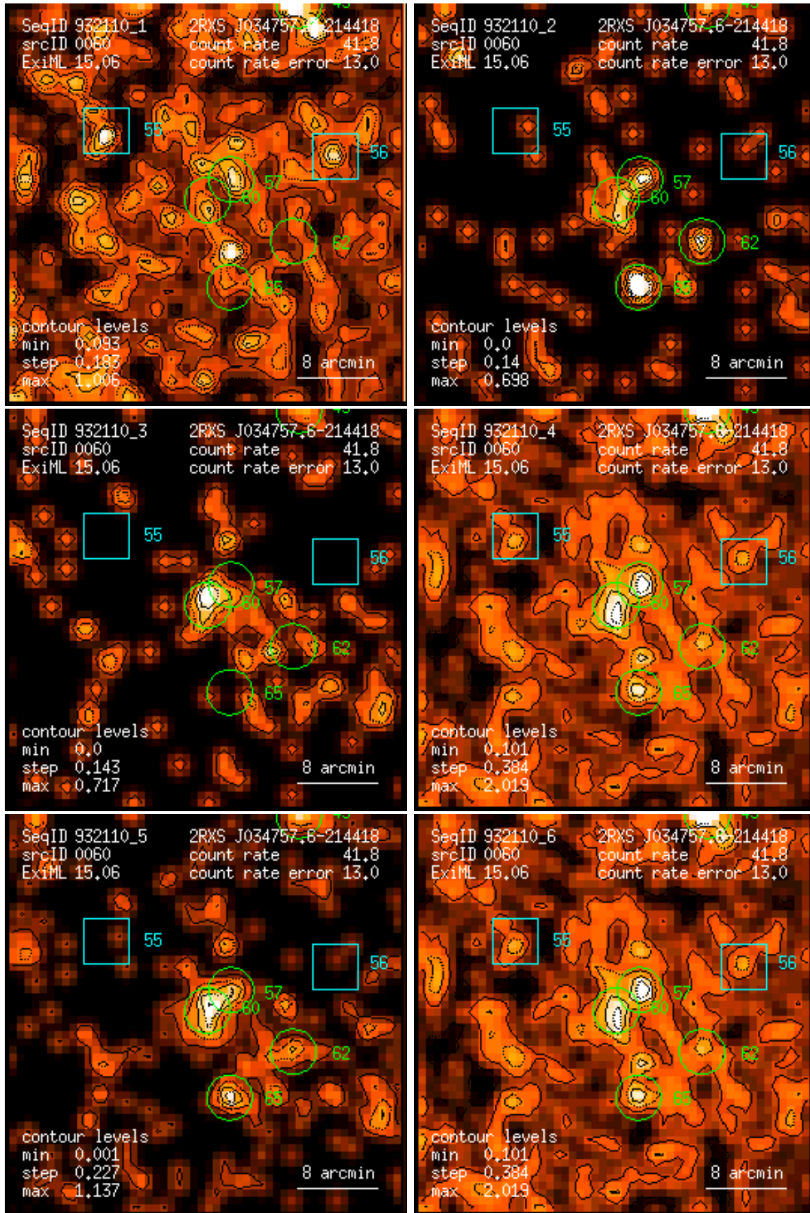
Figure 60: RASS 932110: detection 0060: band rate images, Gaussian filter: (1) PSPC channels 11 – 41, (2) 52 – 90, (3) 91 – 201, (4) 11 – 235, (5) 52 – 201, (6) 11 – 201. Broad band rates in counts/ks. Band rate contour levels in counts/ks/arcmin 2 .
