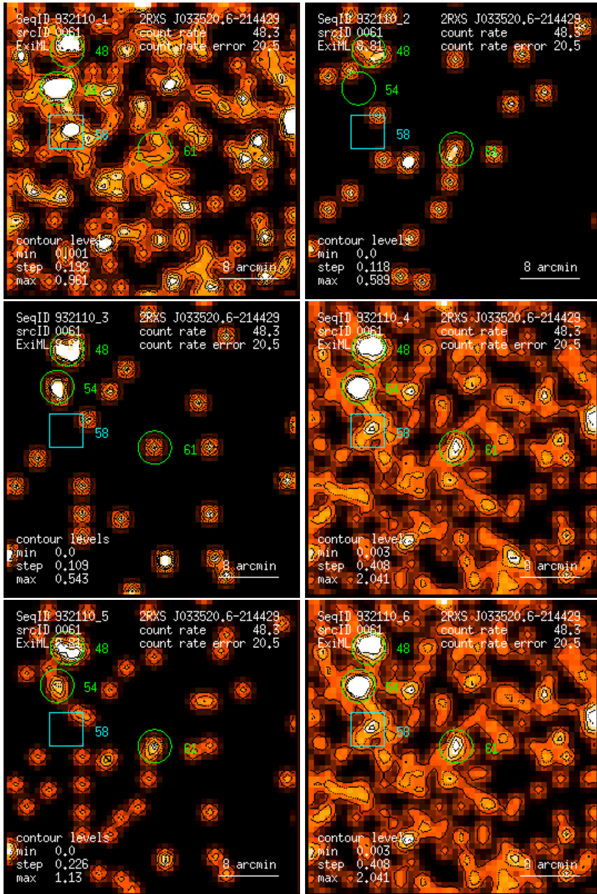
Figure 61: RASS 932110: detection 0061: band rate images, Gaussian filter: (1) PSPC channels 11 – 41, (2) 52 – 90, (3) 91 – 201, (4) 11 – 235, (5) 52 – 201, (6) 11 – 201. Broad band rates in counts/ks. Band rate contour levels in counts/ks/arcmin 2 .
