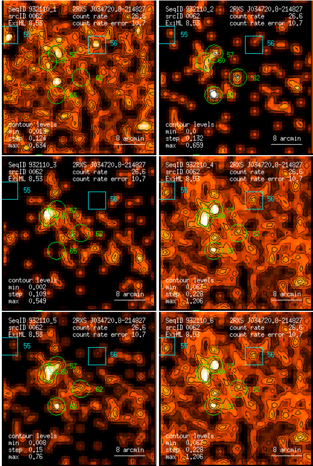
Figure 62: RASS 932110: detection 0062: band rate images, Gaussian filter: (1) PSPC channels 11 – 41, (2) 52 – 90, (3) 91 – 201, (4) 11 – 235, (5) 52 – 201, (6) 11 – 201. Broad band rates in counts/ks. Band rate contour levels in counts/ks/arcmin 2 .
