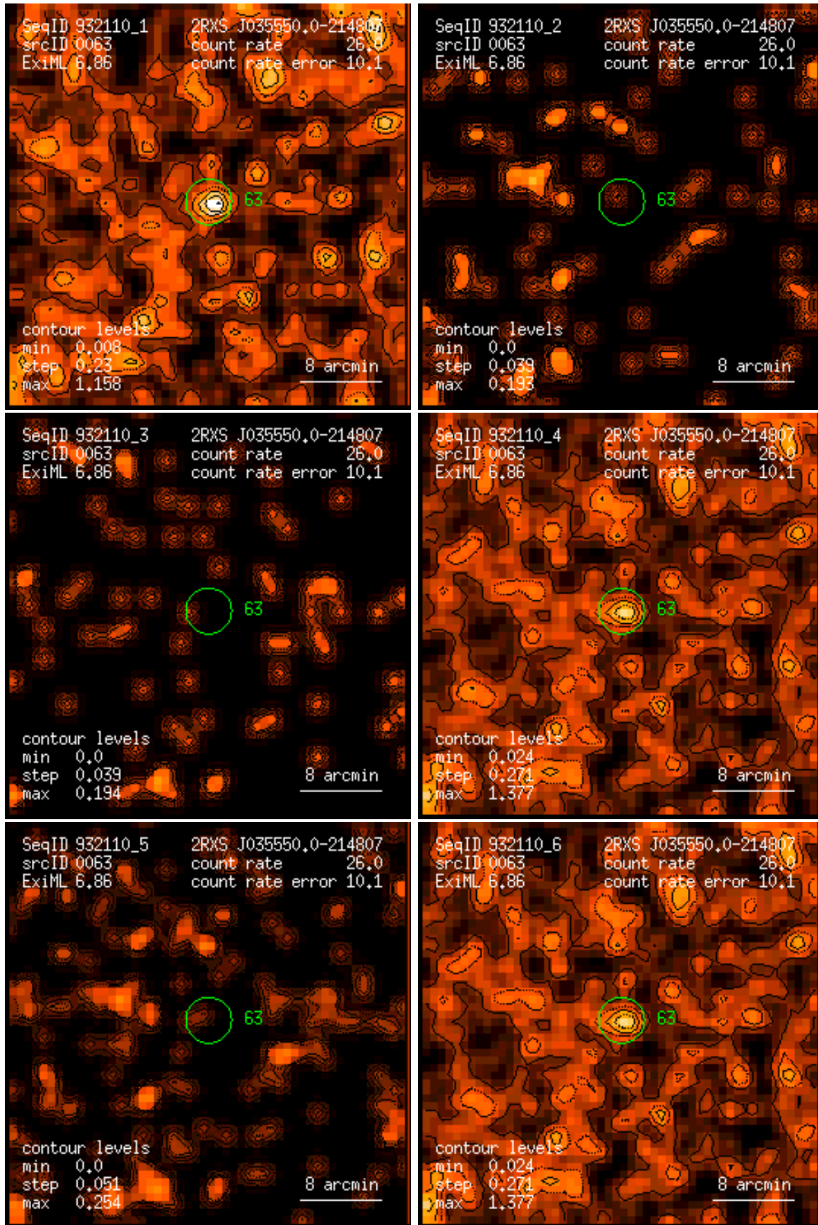
Figure 63: RASS 932110: detection 0063: band rate images, Gaussian filter: (1) PSPC channels 11 – 41, (2) 52 – 90, (3) 91 – 201, (4) 11 – 235, (5) 52 – 201, (6) 11 – 201. Broad band rates in counts/ks. Band rate contour levels in counts/ks/arcmin 2 .
