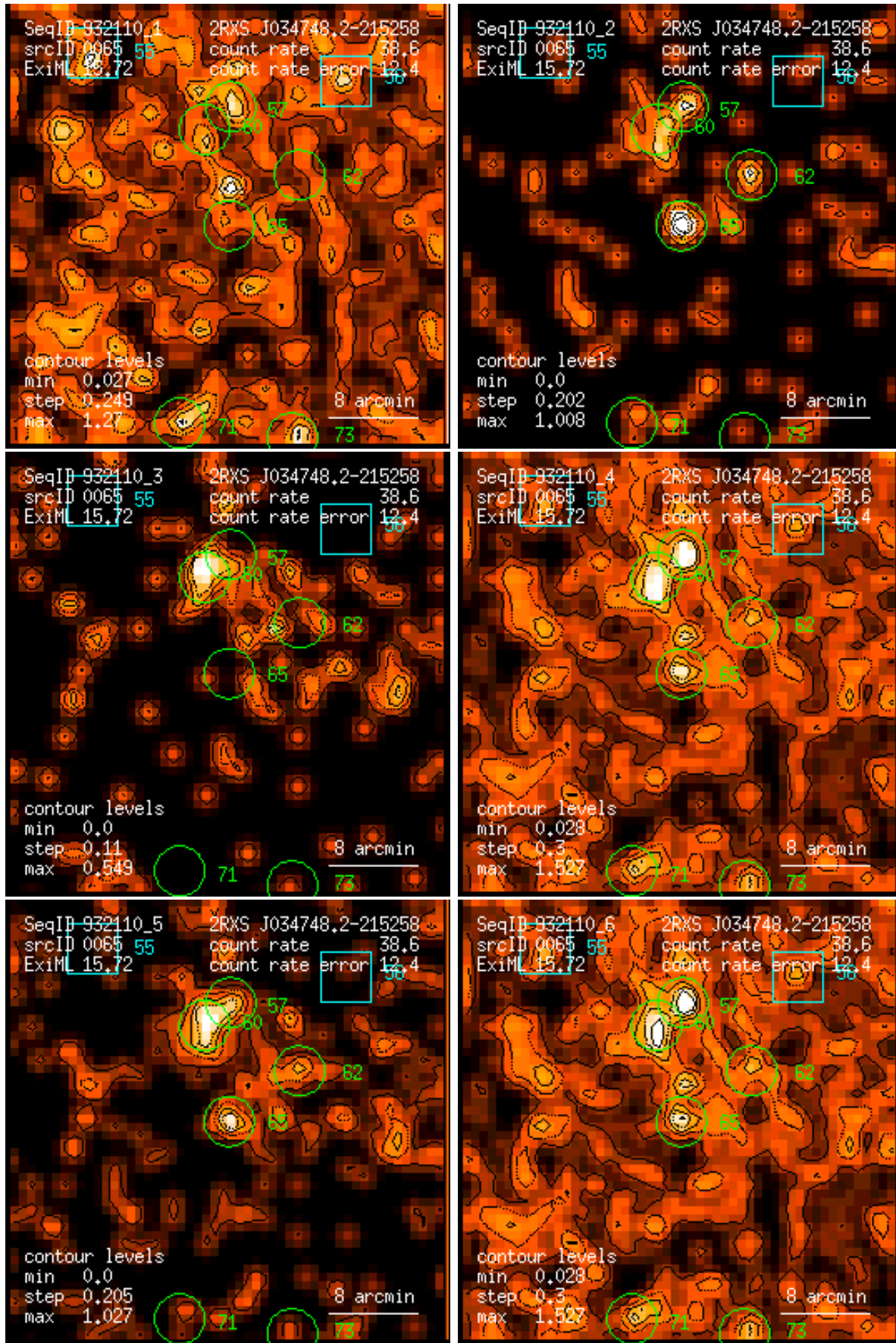
Figure 65: RASS 932110: detection 0065: band rate images, Gaussian filter: (1) PSPC channels 11 – 41, (2) 52 – 90, (3) 91 – 201, (4) 11 – 235, (5) 52 – 201, (6) 11 – 201. Broad band rates in counts/ks. Band rate contour levels in counts/ks/arcmin 2 .
