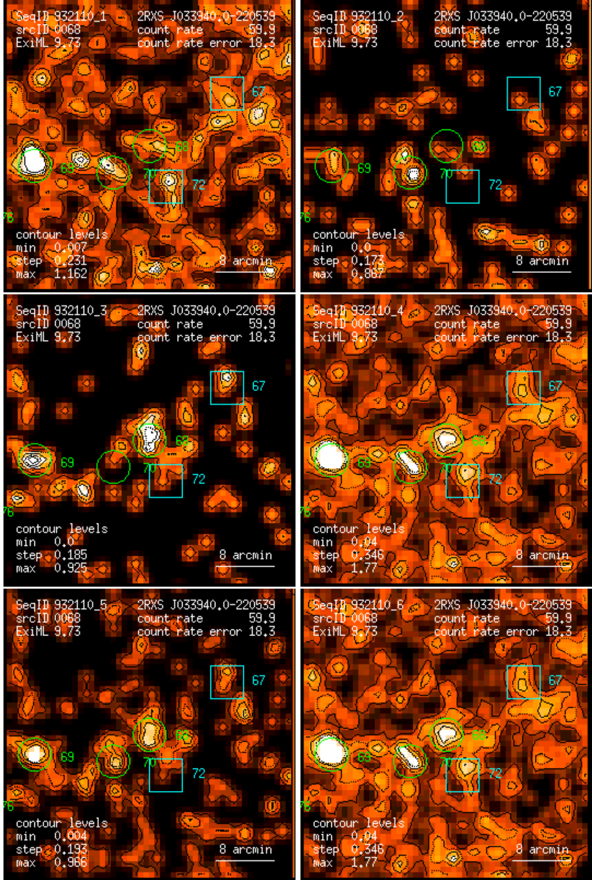
Figure 68: RASS 932110: detection 0068: band rate images, Gaussian filter: (1) PSPC channels 11 – 41, (2) 52 – 90, (3) 91 – 201, (4) 11 – 235, (5) 52 – 201, (6) 11 – 201. Broad band rates in counts/ks. Band rate contour levels in counts/ks/arcmin 2 .
