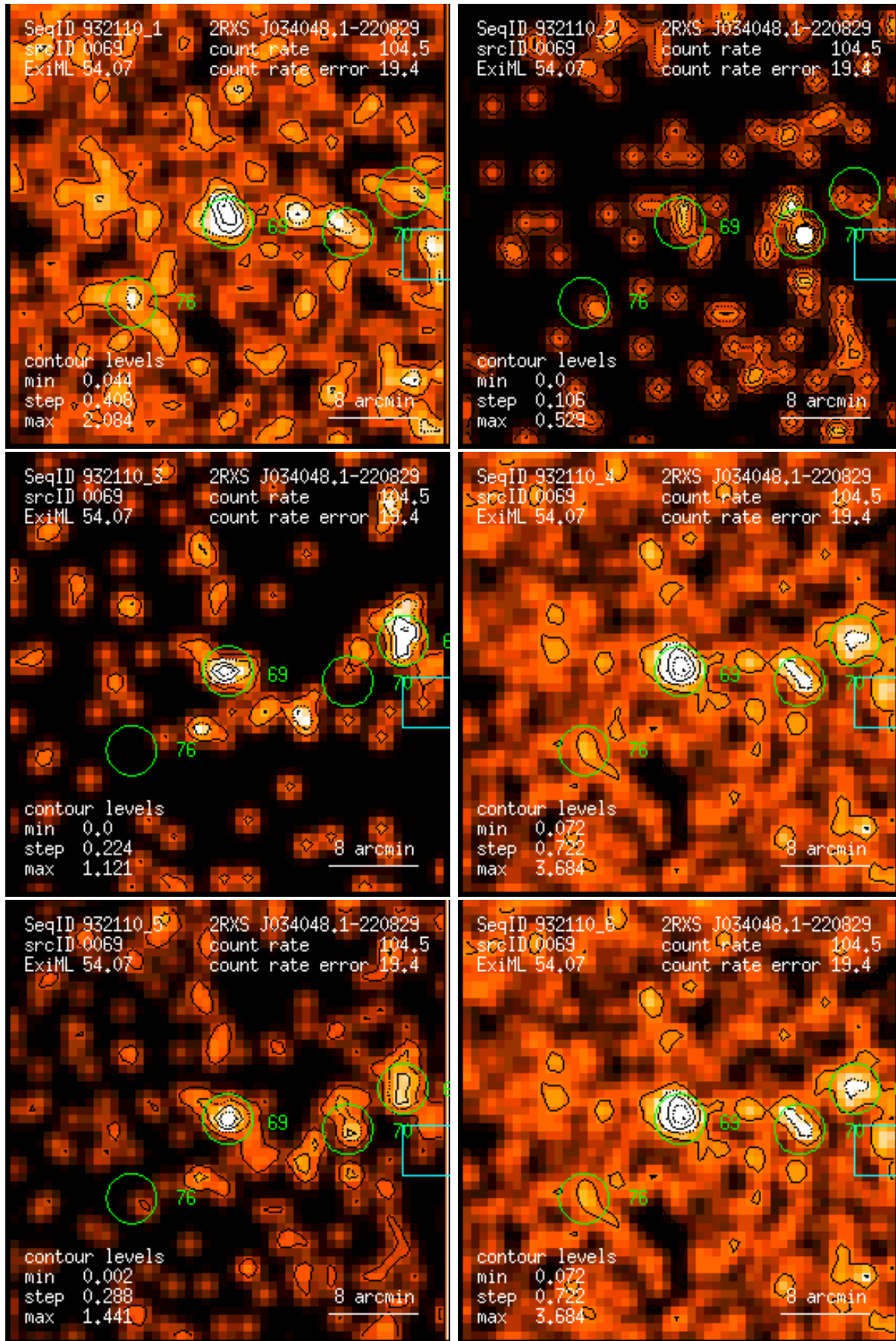
Figure 69: RASS 932110: detection 0069: band rate images, Gaussian filter: (1) PSPC channels 11 – 41, (2) 52 – 90, (3) 91 – 201, (4) 11 – 235, (5) 52 – 201, (6) 11 – 201. Broad band rates in counts/ks. Band rate contour levels in counts/ks/arcmin 2 .
