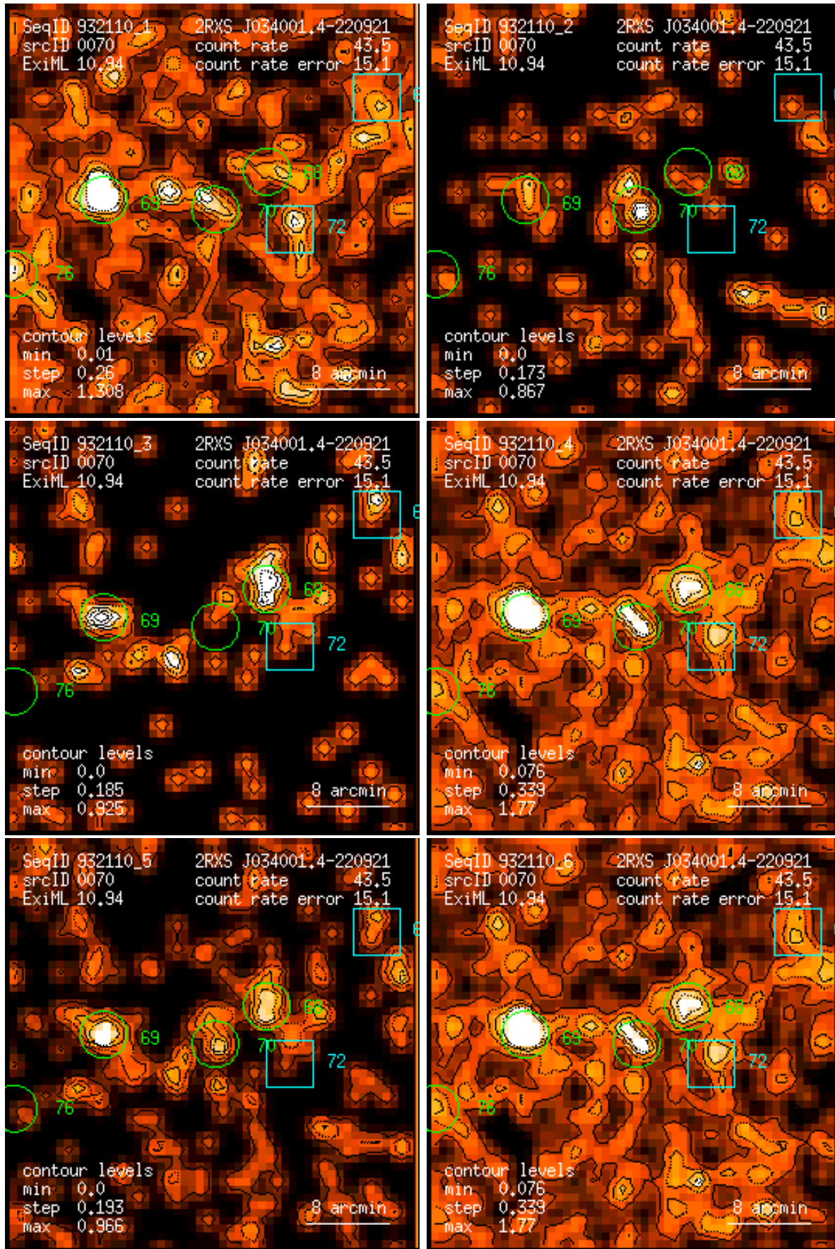
Figure 70: RASS 932110: detection 0070: band rate images, Gaussian filter: (1) PSPC channels 11 – 41, (2) 52 – 90, (3) 91 – 201, (4) 11 – 235, (5) 52 – 201, (6) 11 – 201. Broad band rates in counts/ks. Band rate contour levels in counts/ks/arcmin 2 .
