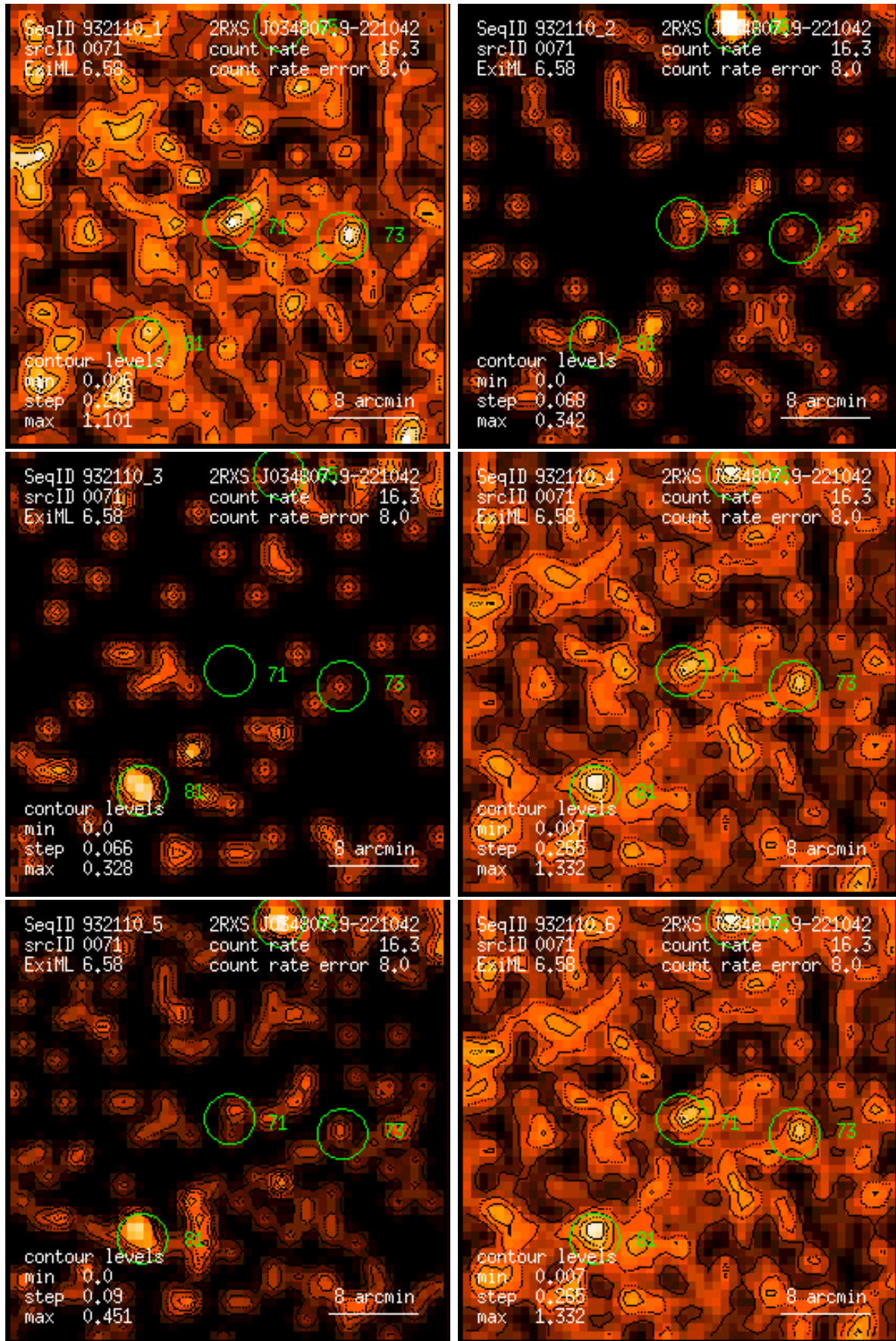
Figure 71: RASS 932110: detection 0071: band rate images, Gaussian filter: (1) PSPC channels 11 – 41, (2) 52 – 90, (3) 91 – 201, (4) 11 – 235, (5) 52 – 201, (6) 11 – 201. Broad band rates in counts/ks. Band rate contour levels in counts/ks/arcmin 2 .
