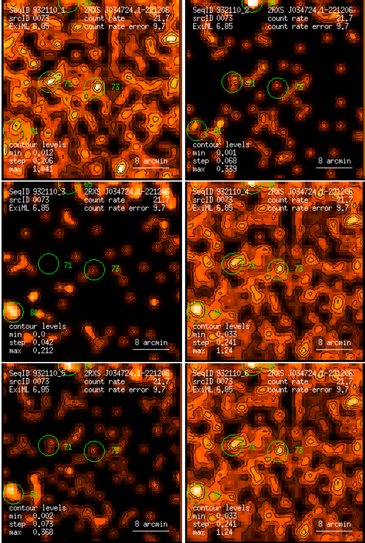
Figure 73: RASS 932110: detection 0073: band rate images, Gaussian filter: (1) PSPC channels 11 – 41, (2) 52 – 90, (3) 91 – 201, (4) 11 – 235, (5) 52 – 201, (6) 11 – 201. Broad band rates in counts/ks. Band rate contour levels in counts/ks/arcmin 2 .
