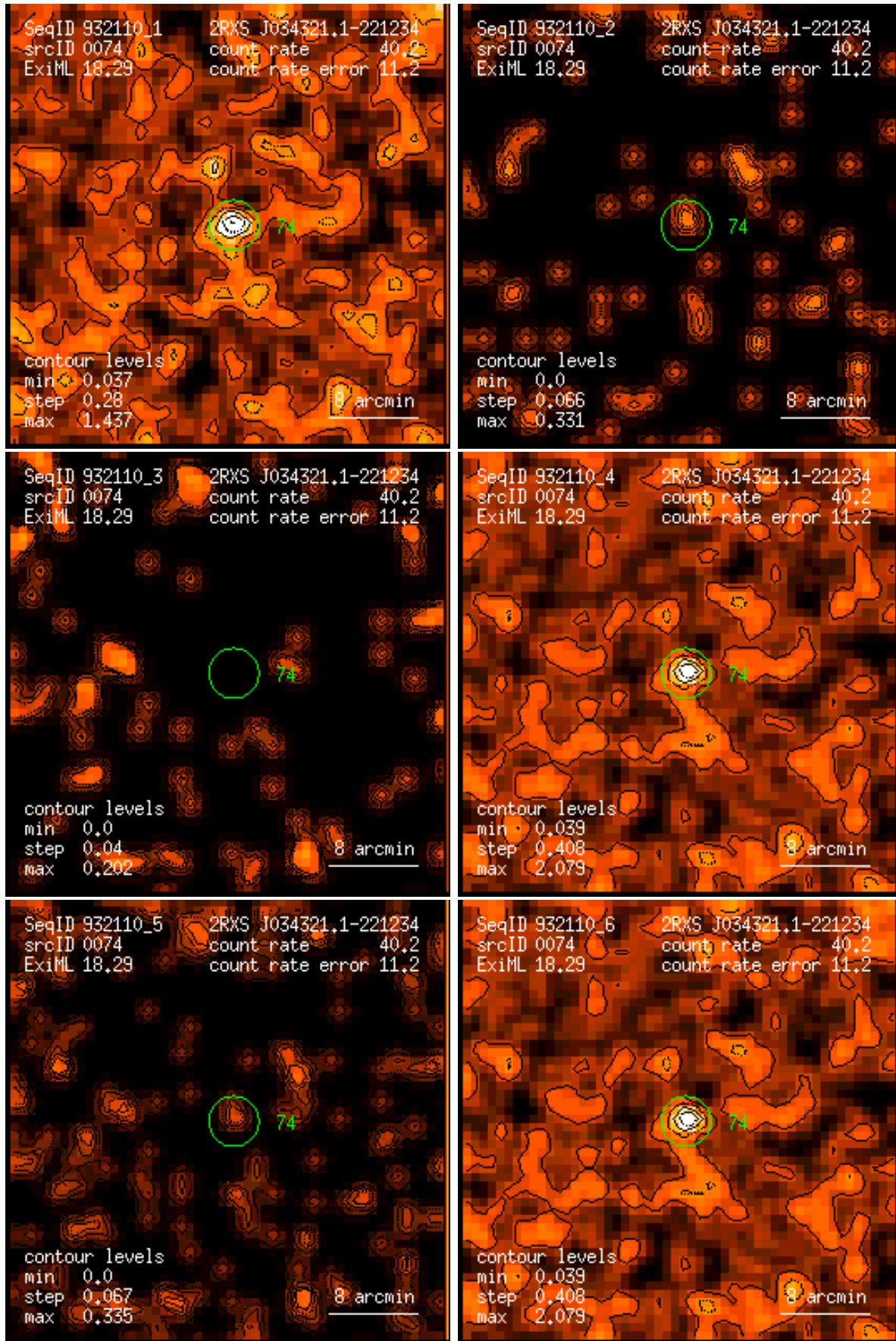
Figure 74: RASS 932110: detection 0074: band rate images, Gaussian filter: (1) PSPC channels 11 – 41, (2) 52 – 90, (3) 91 – 201, (4) 11 – 235, (5) 52 – 201, (6) 11 – 201. Broad band rates in counts/ks. Band rate contour levels in counts/ks/arcmin 2 .
