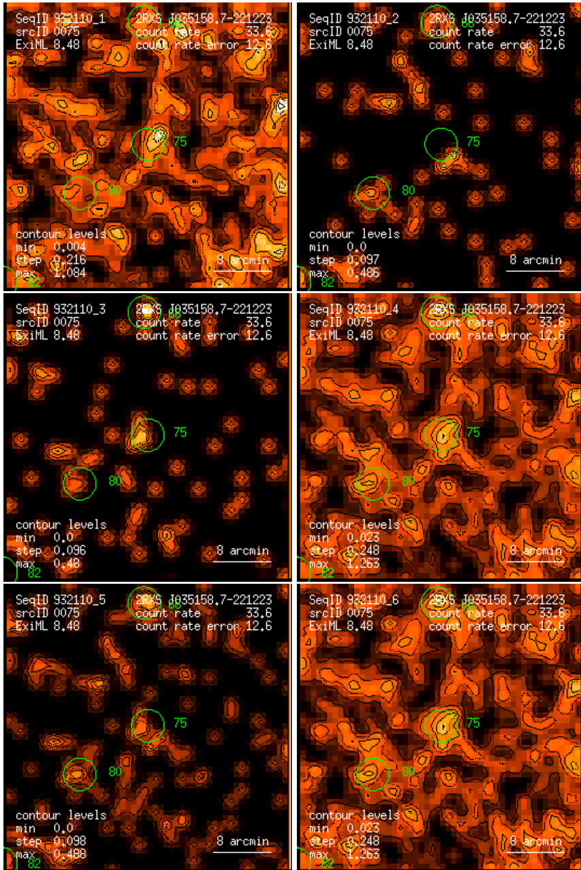
Figure 75: RASS 932110: detection 0075: band rate images, Gaussian filter: (1) PSPC channels 11 – 41, (2) 52 – 90, (3) 91 – 201, (4) 11 – 235, (5) 52 – 201, (6) 11 – 201. Broad band rates in counts/ks. Band rate contour levels in counts/ks/arcmin 2 .
