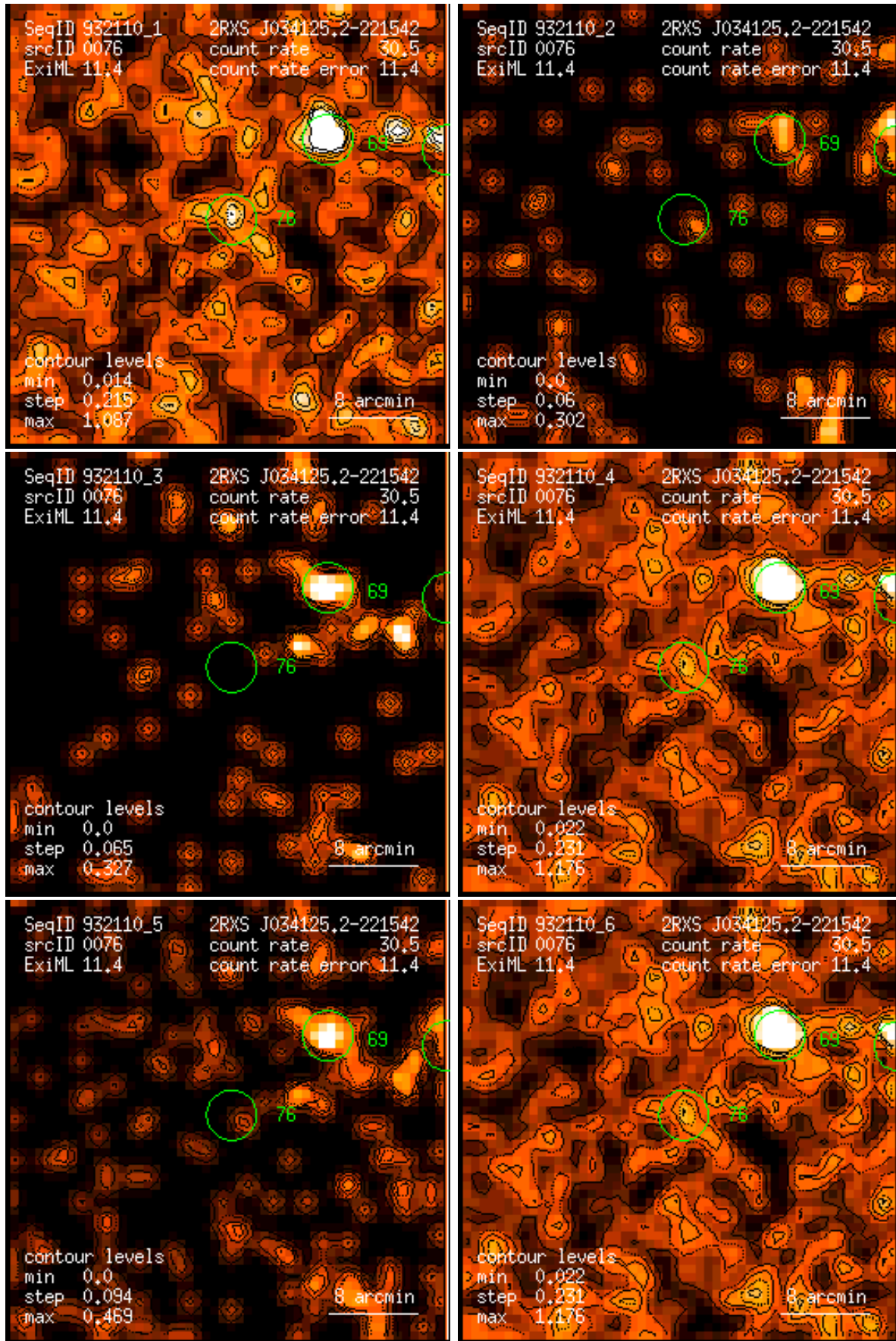
Figure 76: RASS 932110: detection 0076: band rate images, Gaussian filter: (1) PSPC channels 11 – 41, (2) 52 – 90, (3) 91 – 201, (4) 11 – 235, (5) 52 – 201, (6) 11 – 201. Broad band rates in counts/ks. Band rate contour levels in counts/ks/arcmin 2 .
