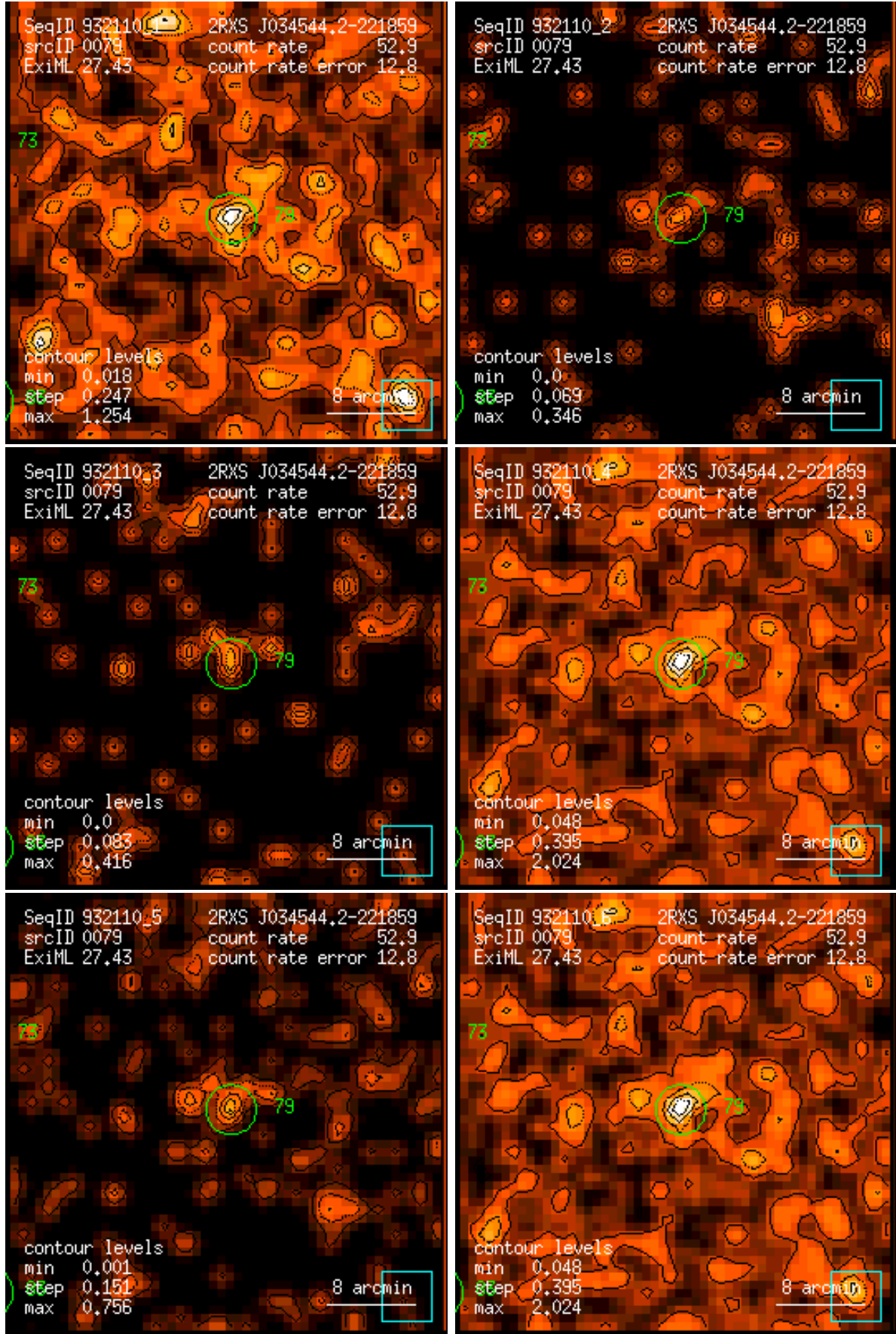
Figure 79: RASS 932110: detection 0079: band rate images, Gaussian filter: (1) PSPC channels 11 – 41, (2) 52 – 90, (3) 91 – 201, (4) 11 – 235, (5) 52 – 201, (6) 11 – 201. Broad band rates in counts/ks. Band rate contour levels in counts/ks/arcmin 2 .
