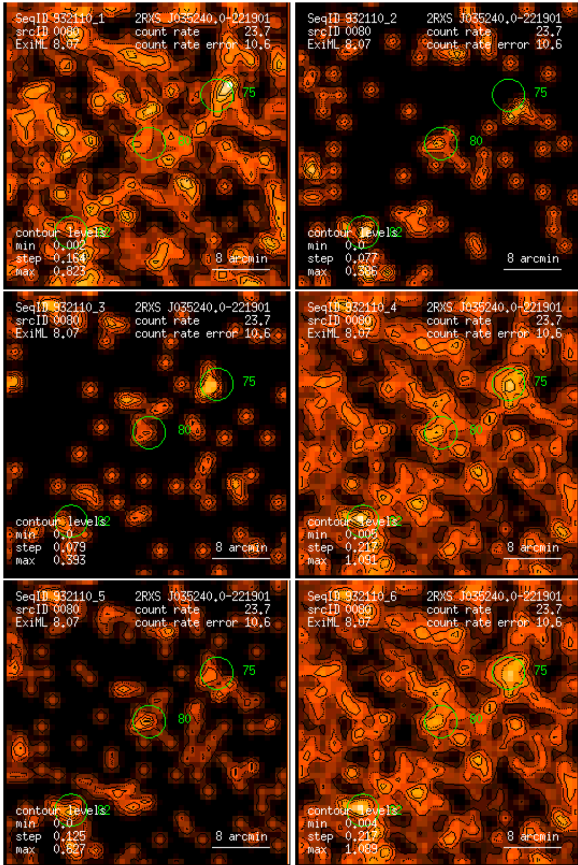
Figure 80: RASS 932110: detection 0080: band rate images, Gaussian filter: (1) PSPC channels 11 – 41, (2) 52 – 90, (3) 91 – 201, (4) 11 – 235, (5) 52 – 201, (6) 11 – 201. Broad band rates in counts/ks. Band rate contour levels in counts/ks/arcmin 2 .
