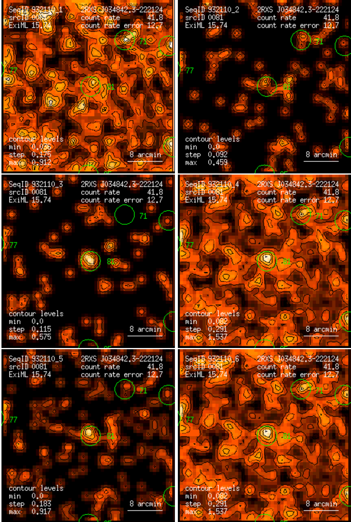
Figure 81: RASS 932110: detection 0081: band rate images, Gaussian filter: (1) PSPC channels 11 – 41, (2) 52 – 90, (3) 91 – 201, (4) 11 – 235, (5) 52 – 201, (6) 11 – 201. Broad band rates in counts/ks. Band rate contour levels in counts/ks/arcmin 2 .
