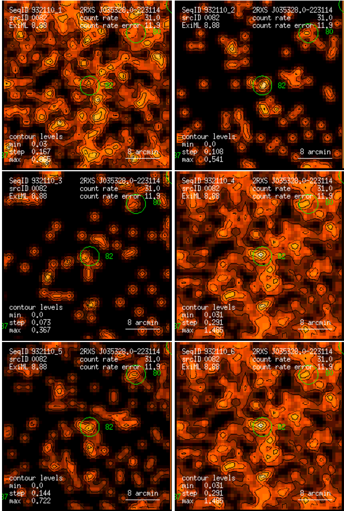
Figure 82: RASS 932110: detection 0082: band rate images, Gaussian filter: (1) PSPC channels 11 – 41, (2) 52 – 90, (3) 91 – 201, (4) 11 – 235, (5) 52 – 201, (6) 11 – 201. Broad band rates in counts/ks. Band rate contour levels in counts/ks/arcmin 2 .
