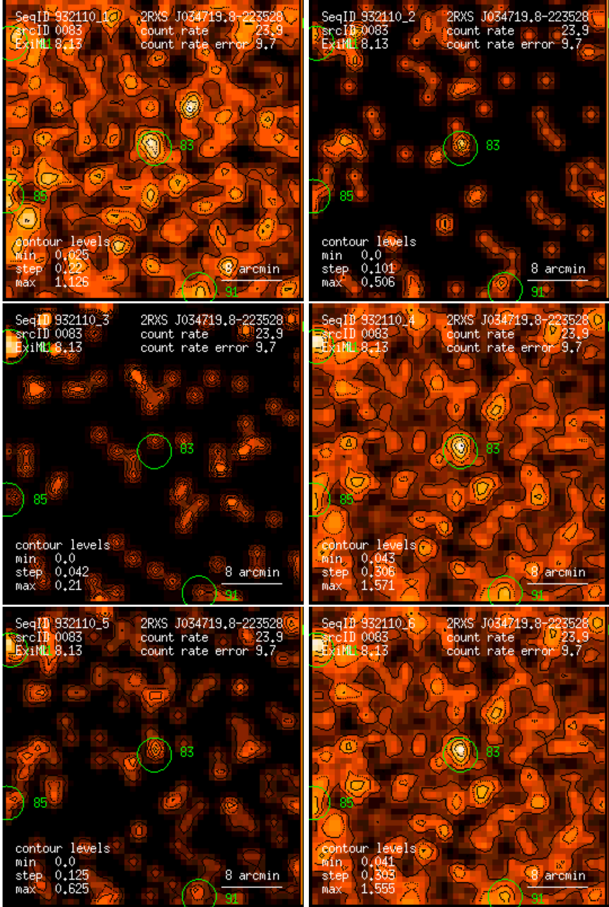
Figure 83: RASS 932110: detection 0083: band rate images, Gaussian filter: (1) PSPC channels 11 – 41, (2) 52 – 90, (3) 91 – 201, (4) 11 – 235, (5) 52 – 201, (6) 11 – 201. Broad band rates in counts/ks. Band rate contour levels in counts/ks/arcmin 2 .
