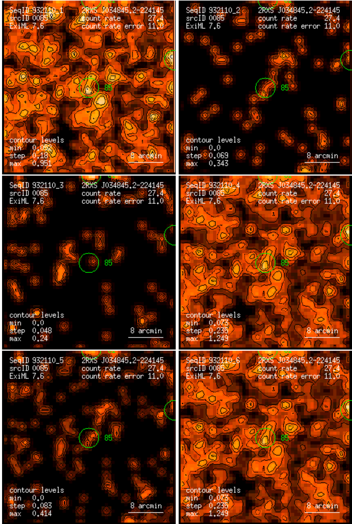
Figure 85: RASS 932110: detection 0085: band rate images, Gaussian filter: (1) PSPC channels 11 – 41, (2) 52 – 90, (3) 91 – 201, (4) 11 – 235, (5) 52 – 201, (6) 11 – 201. Broad band rates in counts/ks. Band rate contour levels in counts/ks/arcmin 2 .
