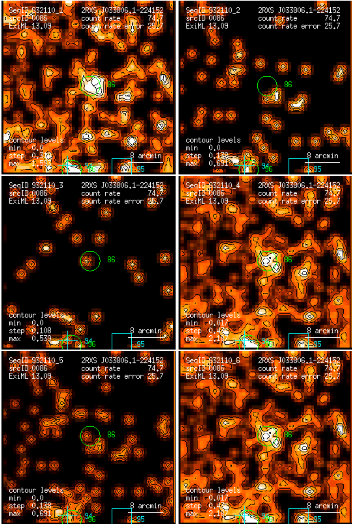
Figure 86: RASS 932110: detection 0086: band rate images, Gaussian filter: (1) PSPC channels 11 – 41, (2) 52 – 90, (3) 91 – 201, (4) 11 – 235, (5) 52 – 201, (6) 11 – 201. Broad band rates in counts/ks. Band rate contour levels in counts/ks/arcmin 2 .
