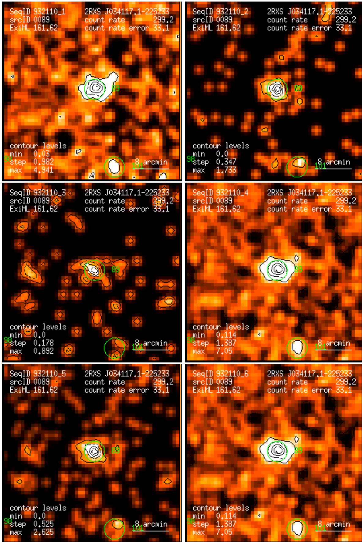
Figure 89: RASS 932110: detection 0089: band rate images, Gaussian filter: (1) PSPC channels 11 – 41, (2) 52 – 90, (3) 91 – 201, (4) 11 – 235, (5) 52 – 201, (6) 11 – 201. Broad band rates in counts/ks. Band rate contour levels in counts/ks/arcmin 2 .
