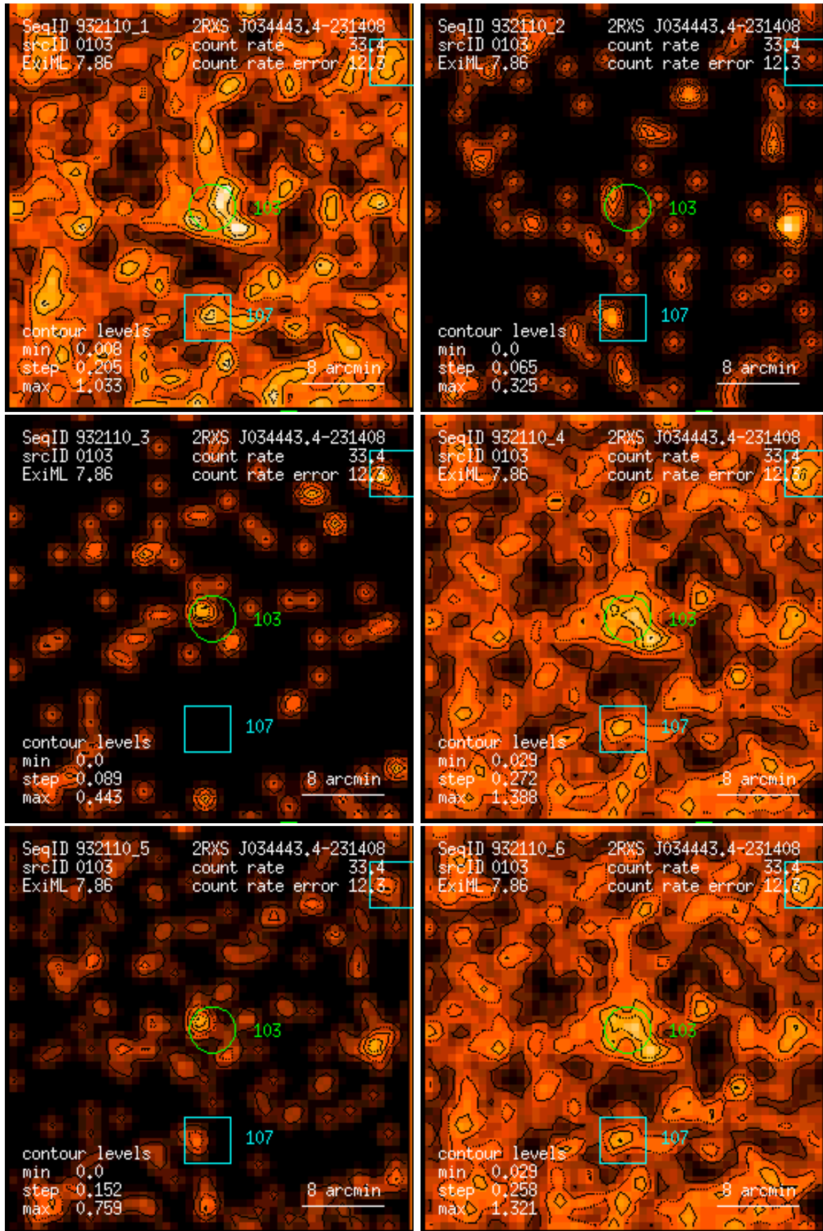
Figure 103: RASS 932110: detection 0103: band rate images, Gaussian filter: (1) PSPC channels 11 – 41, (2) 52 – 90, (3) 91 – 201, (4) 11 – 235, (5) 52 – 201, (6) 11 – 201. Broad band rates in counts/ks. Band rate contour levels in counts/ks/arcmin 2 .
