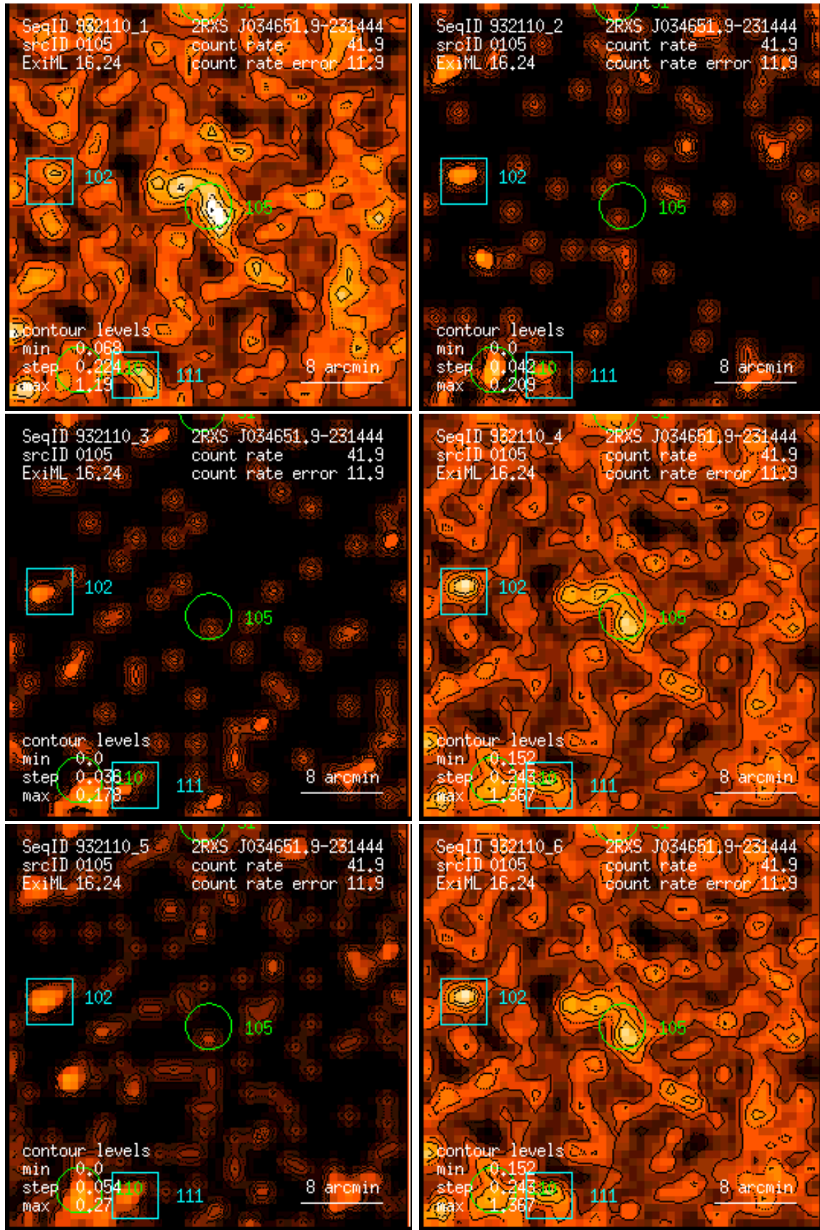
Figure 105: RASS 932110: detection 0105: band rate images, Gaussian filter: (1) PSPC channels 11 – 41, (2) 52 – 90, (3) 91 – 201, (4) 11 – 235, (5) 52 – 201, (6) 11 – 201. Broad band rates in counts/ks. Band rate contour levels in counts/ks/arcmin 2 .
