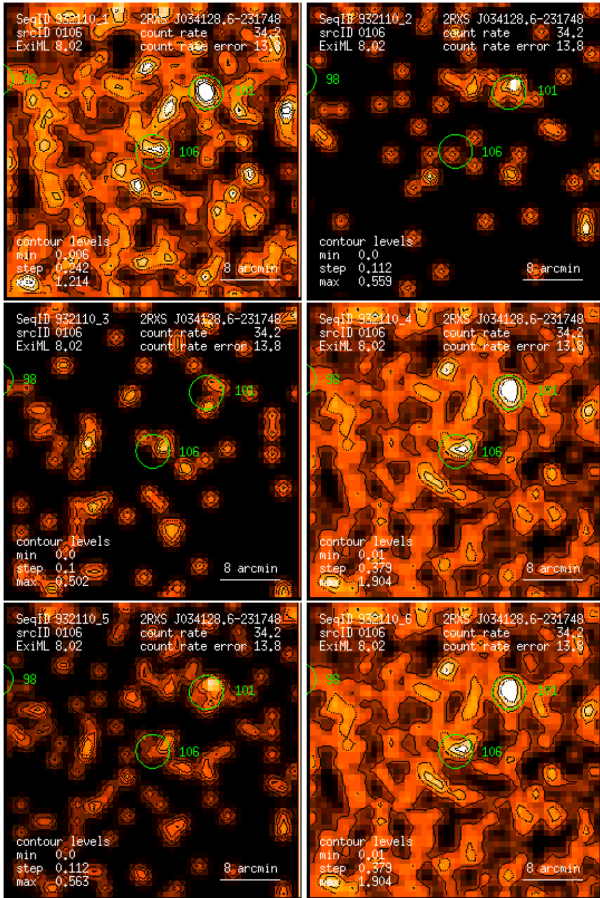
Figure 106: RASS 932110: detection 0106: band rate images, Gaussian filter: (1) PSPC channels 11 – 41, (2) 52 – 90, (3) 91 – 201, (4) 11 – 235, (5) 52 – 201, (6) 11 – 201. Broad band rates in counts/ks. Band rate contour levels in counts/ks/arcmin 2 .
