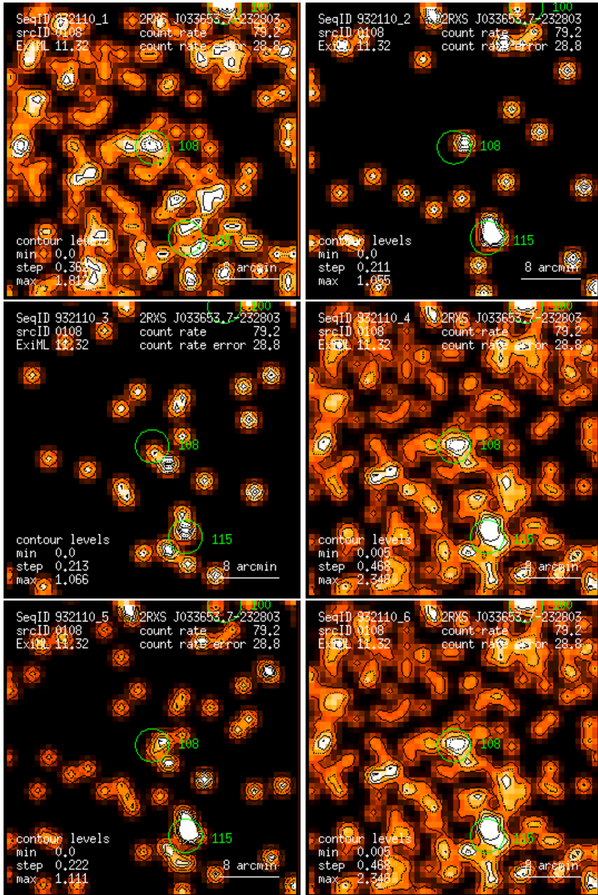
Figure 108: RASS 932110: detection 0108: band rate images, Gaussian filter: (1) PSPC channels 11 – 41, (2) 52 – 90, (3) 91 – 201, (4) 11 – 235, (5) 52 – 201, (6) 11 – 201. Broad band rates in counts/ks. Band rate contour levels in counts/ks/arcmin 2 .
