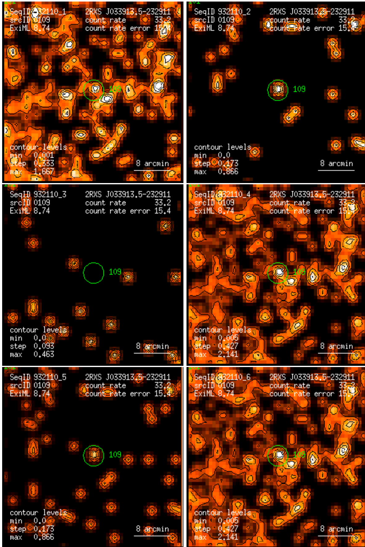
Figure 109: RASS 932110: detection 0109: band rate images, Gaussian filter: (1) PSPC channels 11 – 41, (2) 52 – 90, (3) 91 – 201, (4) 11 – 235, (5) 52 – 201, (6) 11 – 201. Broad band rates in counts/ks. Band rate contour levels in counts/ks/arcmin 2 .
