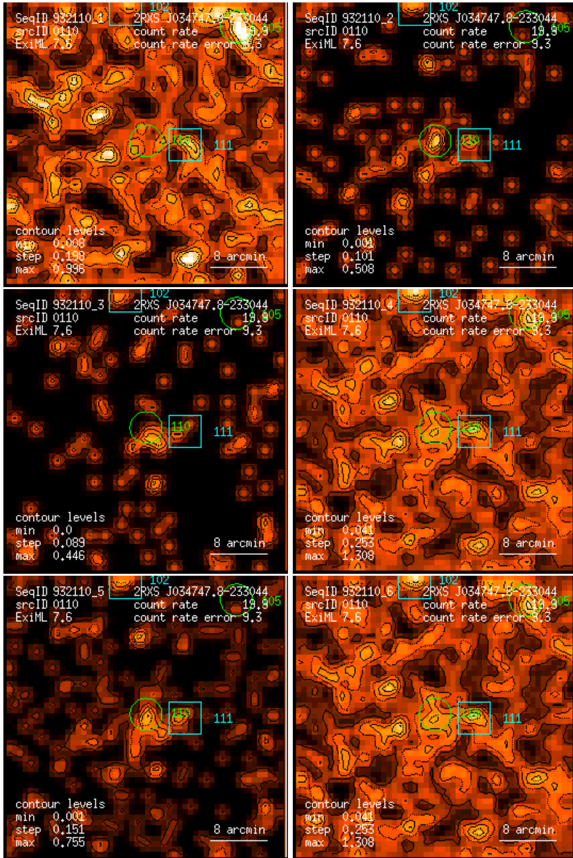
Figure 110: RASS 932110: detection 0110: band rate images, Gaussian filter: (1) PSPC channels 11 – 41, (2) 52 – 90, (3) 91 – 201, (4) 11 – 235, (5) 52 – 201, (6) 11 – 201. Broad band rates in counts/ks. Band rate contour levels in counts/ks/arcmin 2 .
