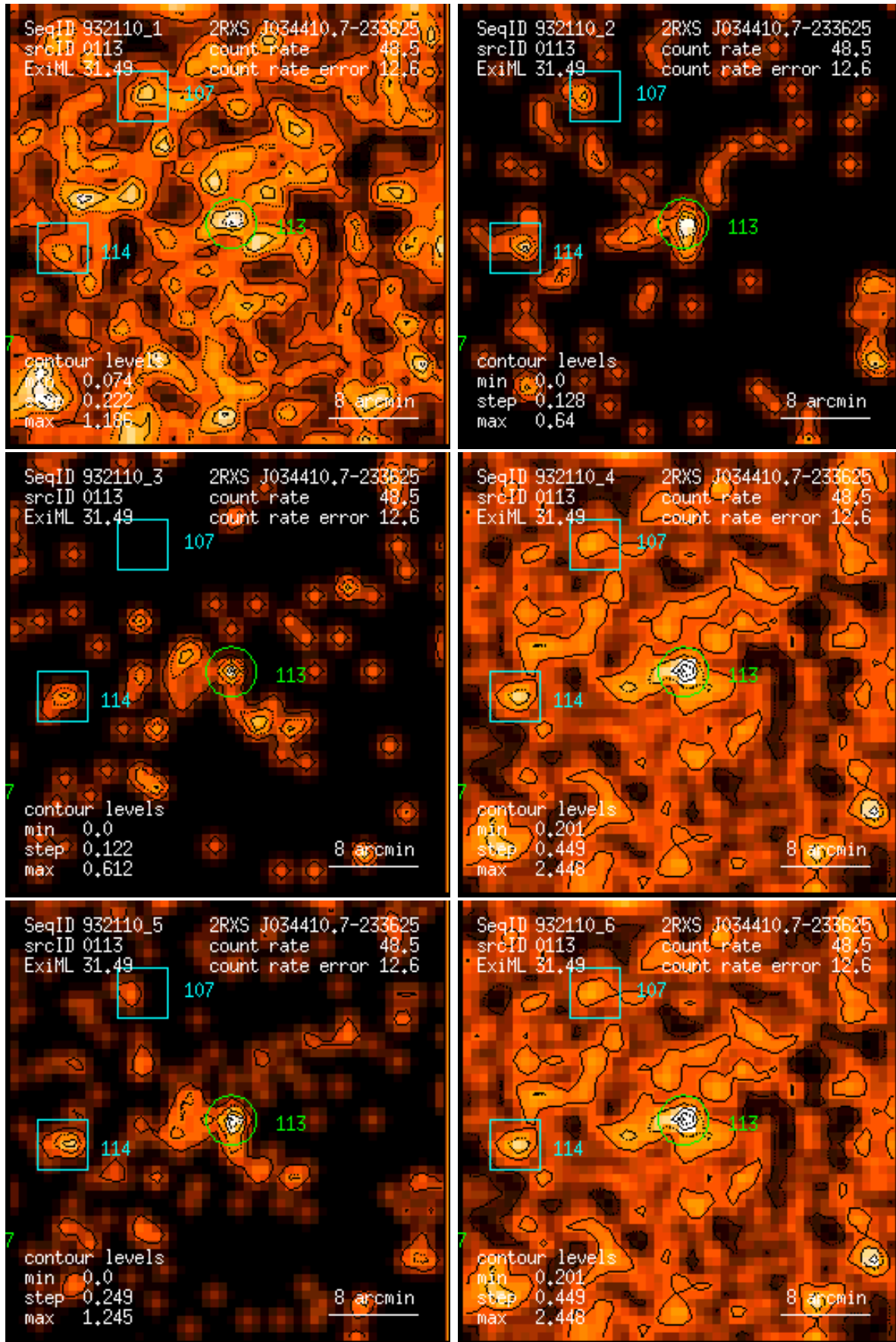
Figure 113: RASS 932110: detection 0113: band rate images, Gaussian filter: (1) PSPC channels 11 – 41, (2) 52 – 90, (3) 91 – 201, (4) 11 – 235, (5) 52 – 201, (6) 11 – 201. Broad band rates in counts/ks. Band rate contour levels in counts/ks/arcmin 2 .
