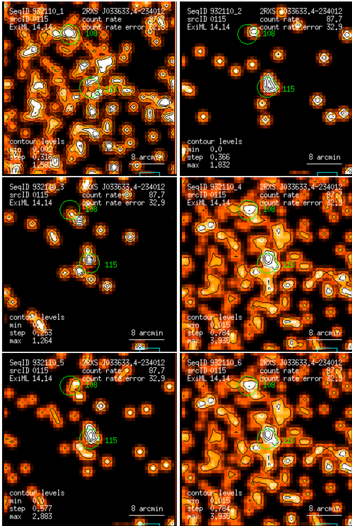
Figure 115: RASS 932110: detection 0115: band rate images, Gaussian filter: (1) PSPC channels 11 – 41, (2) 52 – 90, (3) 91 – 201, (4) 11 – 235, (5) 52 – 201, (6) 11 – 201. Broad band rates in counts/ks. Band rate contour levels in counts/ks/arcmin 2 .
