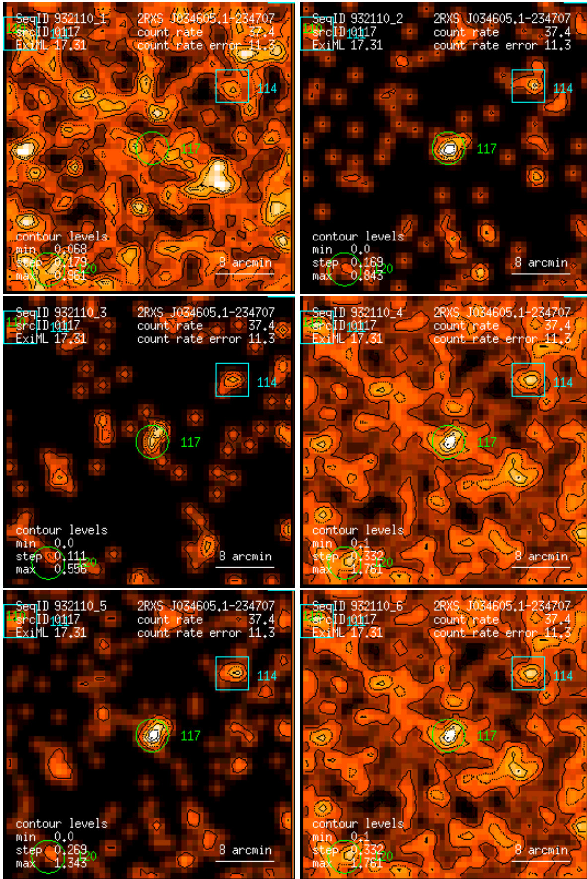
Figure 117: RASS 932110: detection 0117: band rate images, Gaussian filter: (1) PSPC channels 11 – 41, (2) 52 – 90, (3) 91 – 201, (4) 11 – 235, (5) 52 – 201, (6) 11 – 201. Broad band rates in counts/ks. Band rate contour levels in counts/ks/arcmin 2 .
