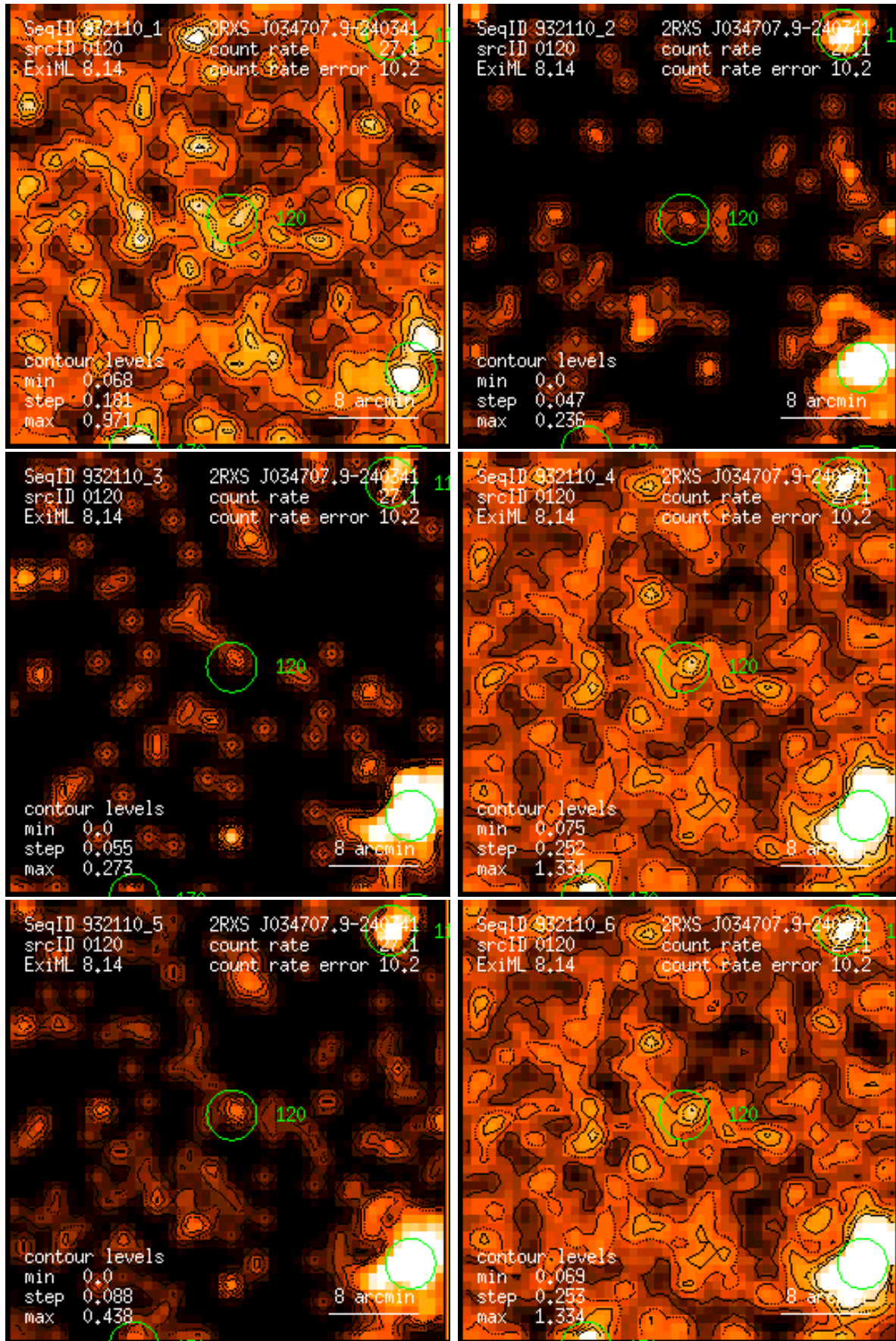
Figure 120: RASS 932110: detection 0120: band rate images, Gaussian filter: (1) PSPC channels 11 – 41, (2) 52 – 90, (3) 91 – 201, (4) 11 – 235, (5) 52 – 201, (6) 11 – 201. Broad band rates in counts/ks. Band rate contour levels in counts/ks/arcmin 2 .
