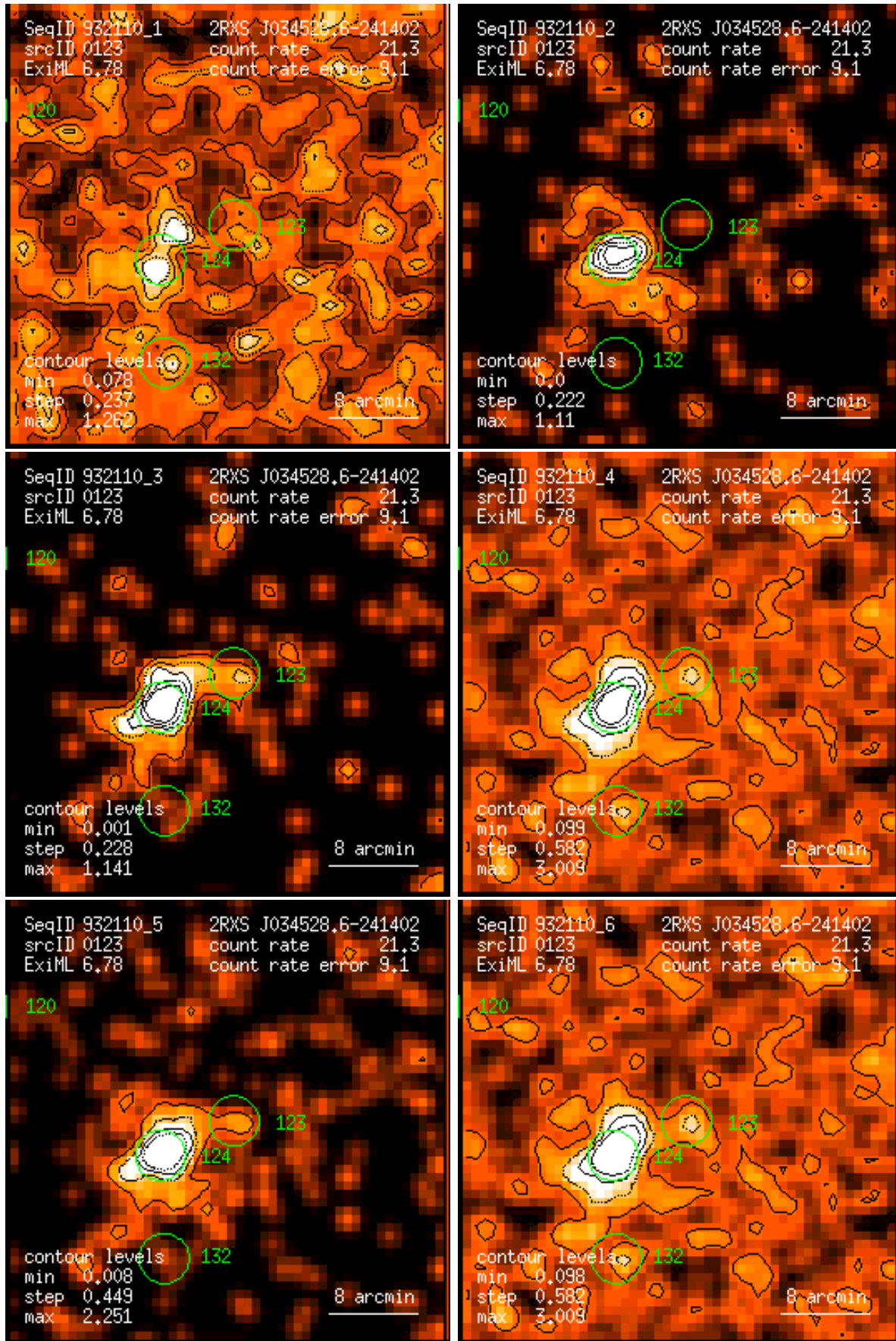
Figure 123: RASS 932110: detection 0123: band rate images, Gaussian filter: (1) PSPC channels 11 – 41, (2) 52 – 90, (3) 91 – 201, (4) 11 – 235, (5) 52 – 201, (6) 11 – 201. Broad band rates in counts/ks. Band rate contour levels in counts/ks/arcmin 2 .
