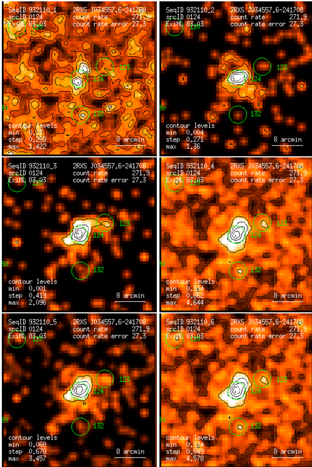
Figure 124: RASS 932110: detection 0124: band rate images, Gaussian filter: (1) PSPC channels 11 – 41, (2) 52 – 90, (3) 91 – 201, (4) 11 – 235, (5) 52 – 201, (6) 11 – 201. Broad band rates in counts/ks. Band rate contour levels in counts/ks/arcmin 2 .
