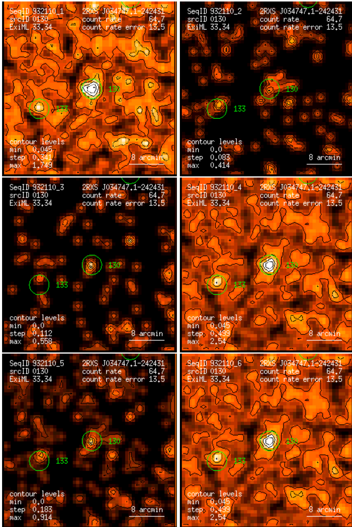
Figure 130: RASS 932110: detection 0130: band rate images, Gaussian filter: (1) PSPC channels 11 – 41, (2) 52 – 90, (3) 91 – 201, (4) 11 – 235, (5) 52 – 201, (6) 11 – 201. Broad band rates in counts/ks. Band rate contour levels in counts/ks/arcmin 2 .
