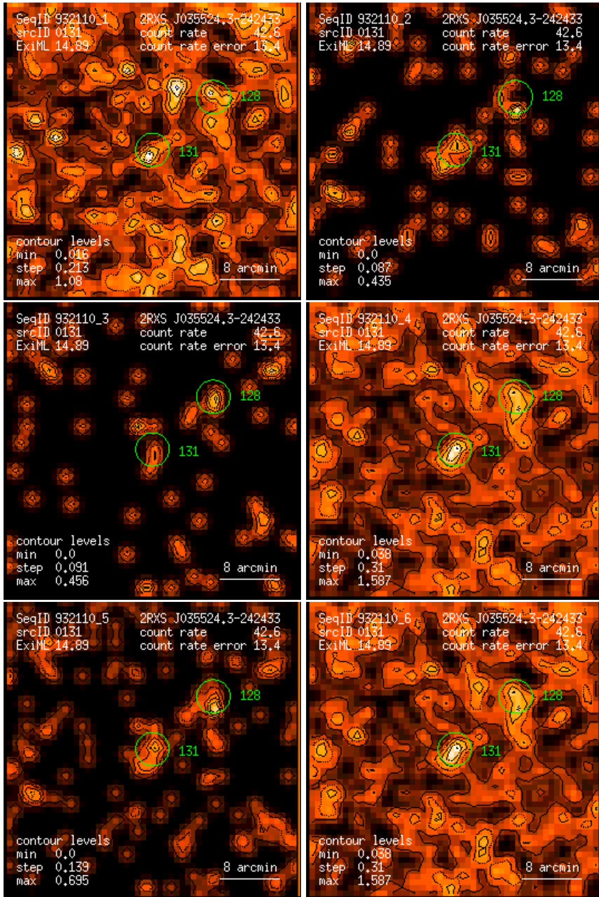
Figure 131: RASS 932110: detection 0131: band rate images, Gaussian filter: (1) PSPC channels 11 – 41, (2) 52 – 90, (3) 91 – 201, (4) 11 – 235, (5) 52 – 201, (6) 11 – 201. Broad band rates in counts/ks. Band rate contour levels in counts/ks/arcmin 2 .
