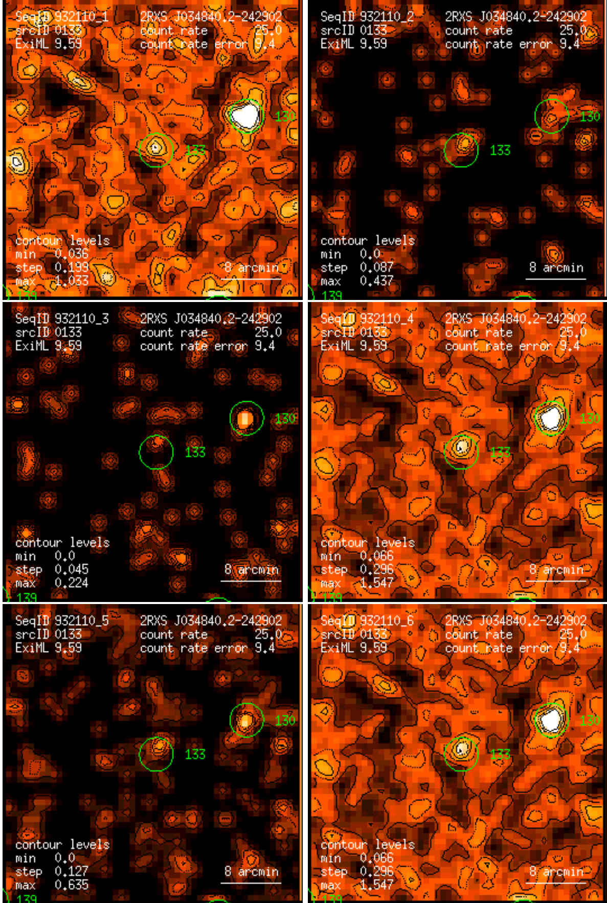
Figure 133: RASS 932110: detection 0133: band rate images, Gaussian filter: (1) PSPC channels 11 – 41, (2) 52 – 90, (3) 91 – 201, (4) 11 – 235, (5) 52 – 201, (6) 11 – 201. Broad band rates in counts/ks. Band rate contour levels in counts/ks/arcmin 2 .
