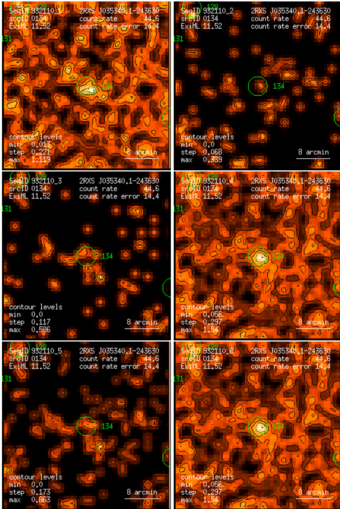
Figure 134: RASS 932110: detection 0134: band rate images, Gaussian filter: (1) PSPC channels 11 – 41, (2) 52 – 90, (3) 91 – 201, (4) 11 – 235, (5) 52 – 201, (6) 11 – 201. Broad band rates in counts/ks. Band rate contour levels in counts/ks/arcmin 2 .
