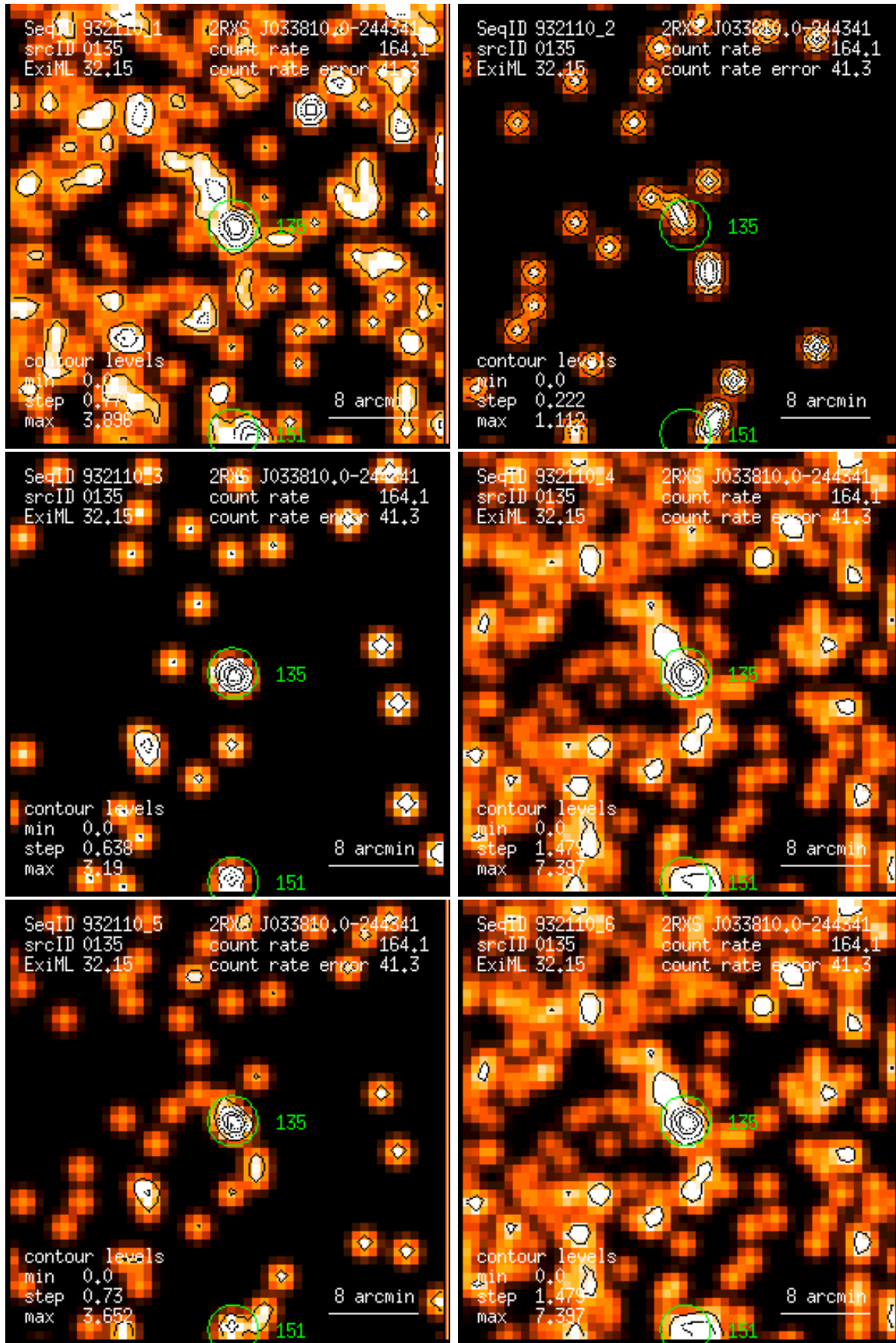
Figure 135: RASS 932110: detection 0135: band rate images, Gaussian filter: (1) PSPC channels 11 – 41, (2) 52 – 90, (3) 91 – 201, (4) 11 – 235, (5) 52 – 201, (6) 11 – 201. Broad band rates in counts/ks. Band rate contour levels in counts/ks/arcmin 2 .
