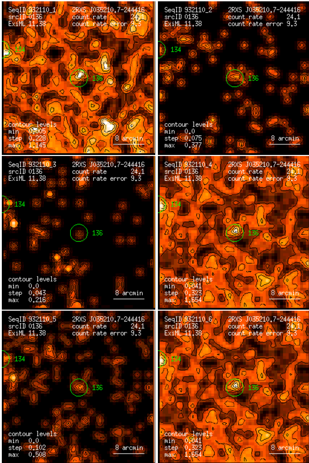
Figure 136: RASS 932110: detection 0136: band rate images, Gaussian filter: (1) PSPC channels 11 – 41, (2) 52 – 90, (3) 91 – 201, (4) 11 – 235, (5) 52 – 201, (6) 11 – 201. Broad band rates in counts/ks. Band rate contour levels in counts/ks/arcmin 2 .
