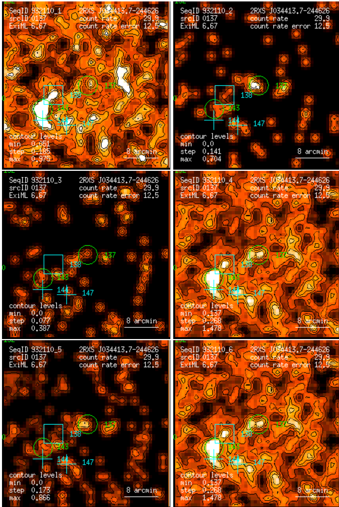
Figure 137: RASS 932110: detection 0137: band rate images, Gaussian filter: (1) PSPC channels 11 – 41, (2) 52 – 90, (3) 91 – 201, (4) 11 – 235, (5) 52 – 201, (6) 11 – 201. Broad band rates in counts/ks. Band rate contour levels in counts/ks/arcmin 2 .
