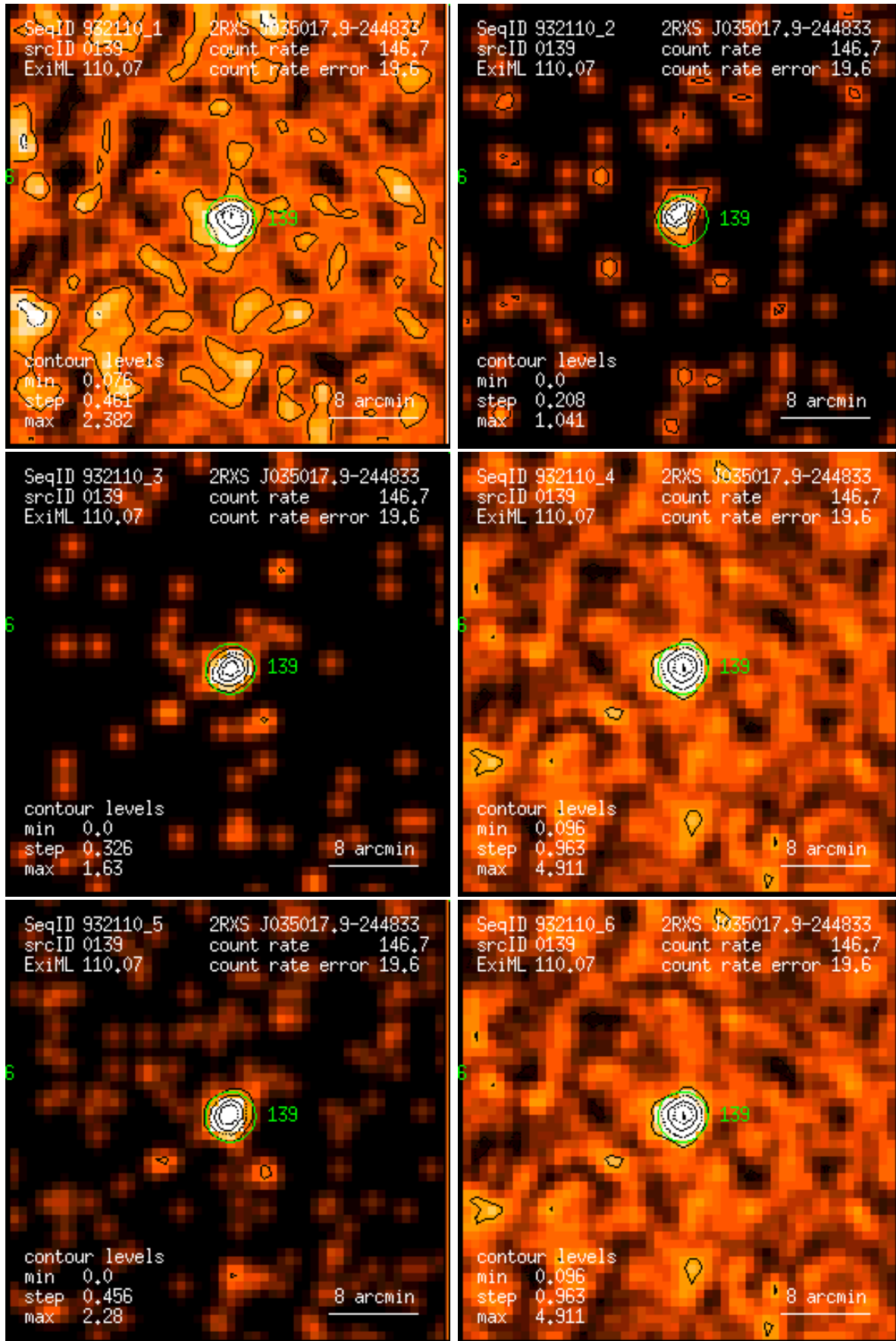
Figure 139: RASS 932110: detection 0139: band rate images, Gaussian filter: (1) PSPC channels 11 – 41, (2) 52 – 90, (3) 91 – 201, (4) 11 – 235, (5) 52 – 201, (6) 11 – 201. Broad band rates in counts/ks. Band rate contour levels in counts/ks/arcmin 2 .
