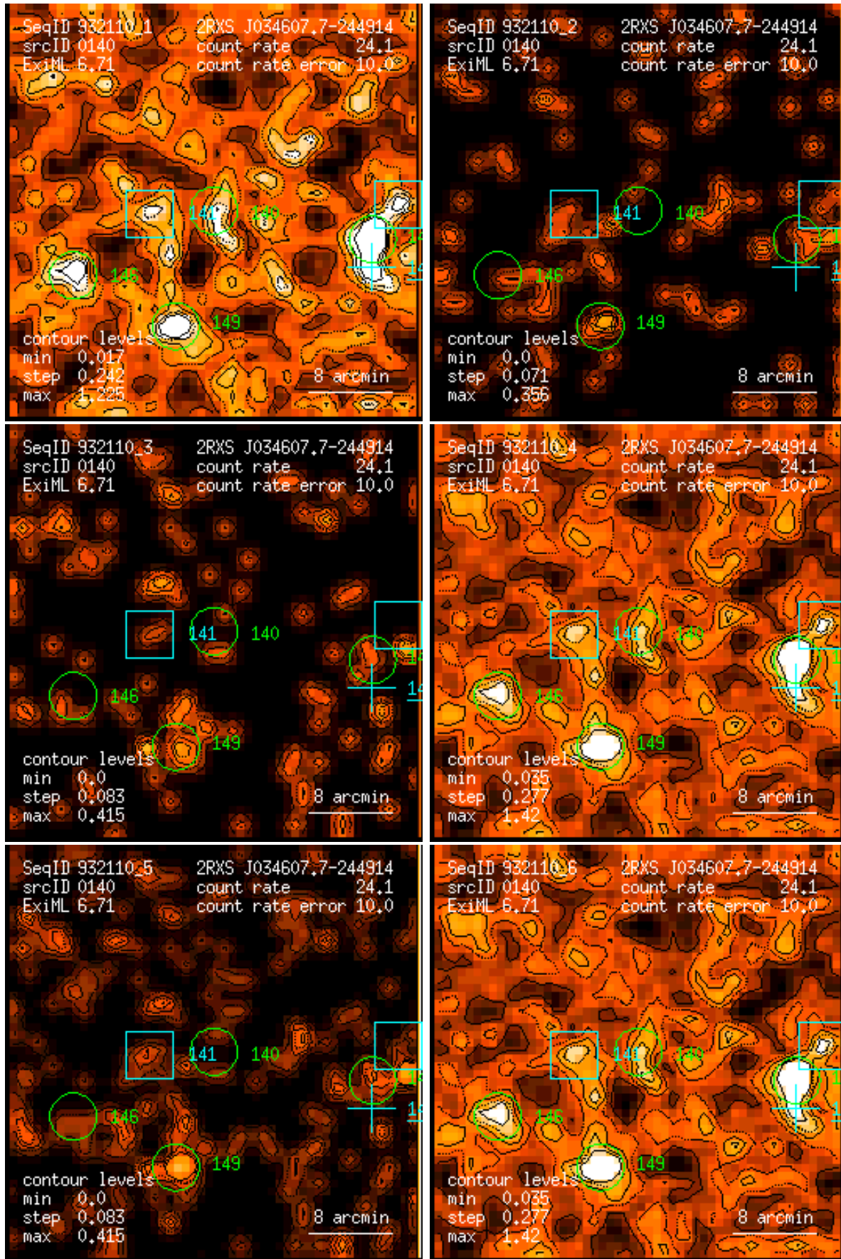
Figure 140: RASS 932110: detection 0140: band rate images, Gaussian filter: (1) PSPC channels 11 – 41, (2) 52 – 90, (3) 91 – 201, (4) 11 – 235, (5) 52 – 201, (6) 11 – 201. Broad band rates in counts/ks. Band rate contour levels in counts/ks/arcmin 2 .
